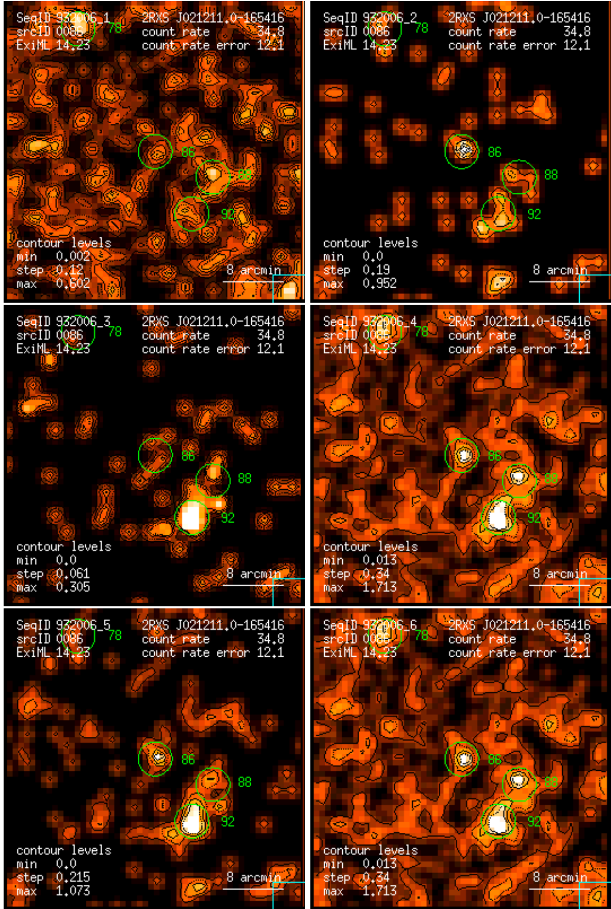
Figure 86: RASS 932006: detection 0086: band rate images, Gaussian filter: (1) PSPC channels 11 – 41, (2) 52 – 90, (3) 91 – 201, (4) 11 – 235, (5) 52 – 201, (6) 11 – 201. Broad band rates in counts/ks. Band rate contour levels in counts/ks/arcmin 2 .
