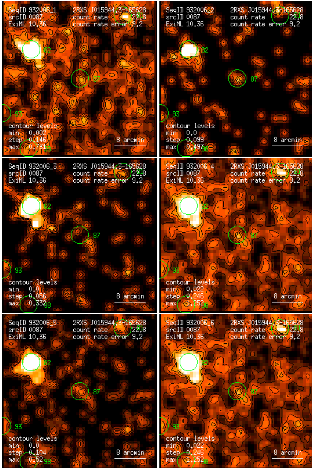
Figure 87: RASS 932006: detection 0087: band rate images, Gaussian filter: (1) PSPC channels 11 – 41, (2) 52 – 90, (3) 91 – 201, (4) 11 – 235, (5) 52 – 201, (6) 11 – 201. Broad band rates in counts/ks. Band rate contour levels in counts/ks/arcmin 2 .
