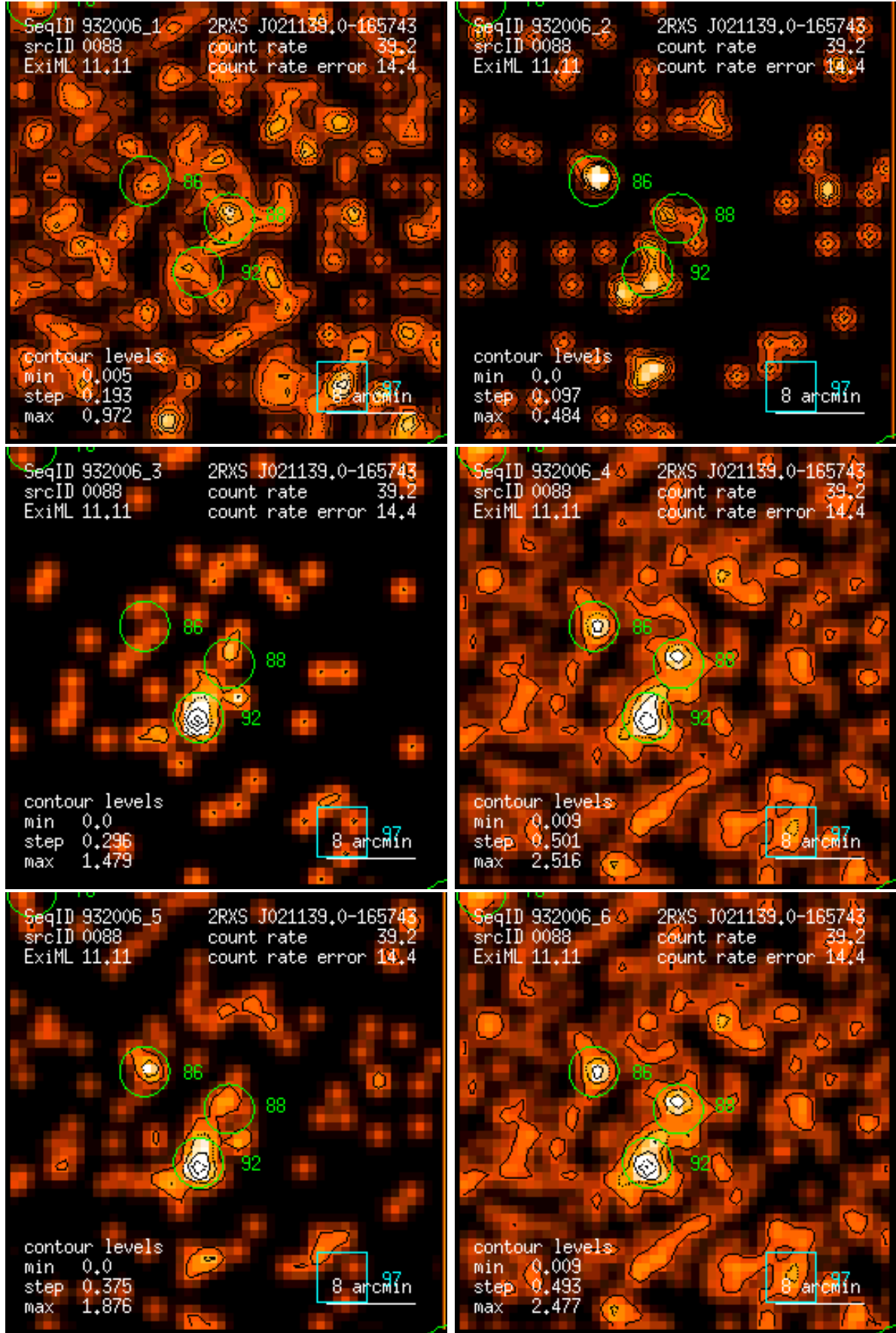
Figure 88: RASS 932006: detection 0088: band rate images, Gaussian filter: (1) PSPC channels 11 – 41, (2) 52 – 90, (3) 91 – 201, (4) 11 – 235, (5) 52 – 201, (6) 11 – 201. Broad band rates in counts/ks. Band rate contour levels in counts/ks/arcmin 2 .
