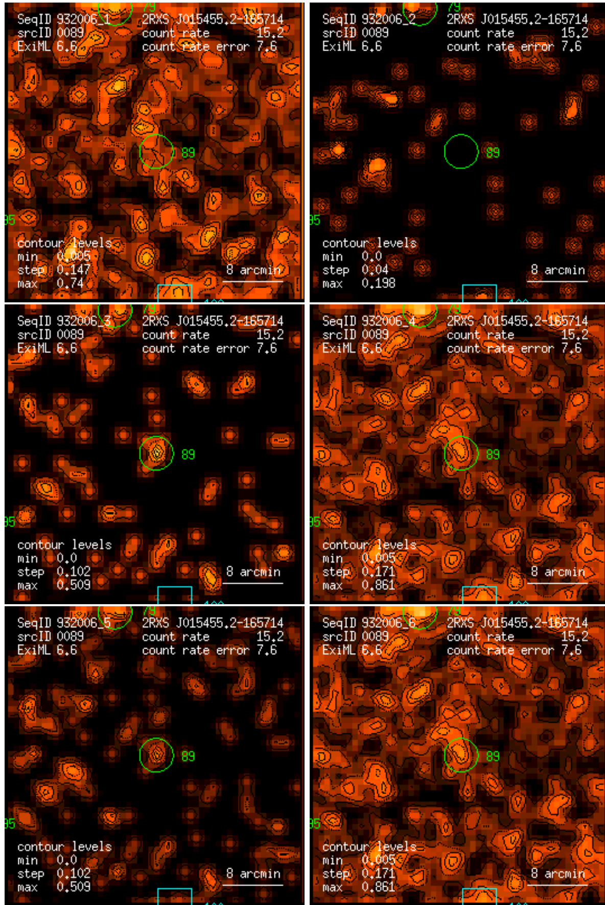
Figure 89: RASS 932006: detection 0089: band rate images, Gaussian filter: (1) PSPC channels 11 – 41, (2) 52 – 90, (3) 91 – 201, (4) 11 – 235, (5) 52 – 201, (6) 11 – 201. Broad band rates in counts/ks. Band rate contour levels in counts/ks/arcmin 2 .
