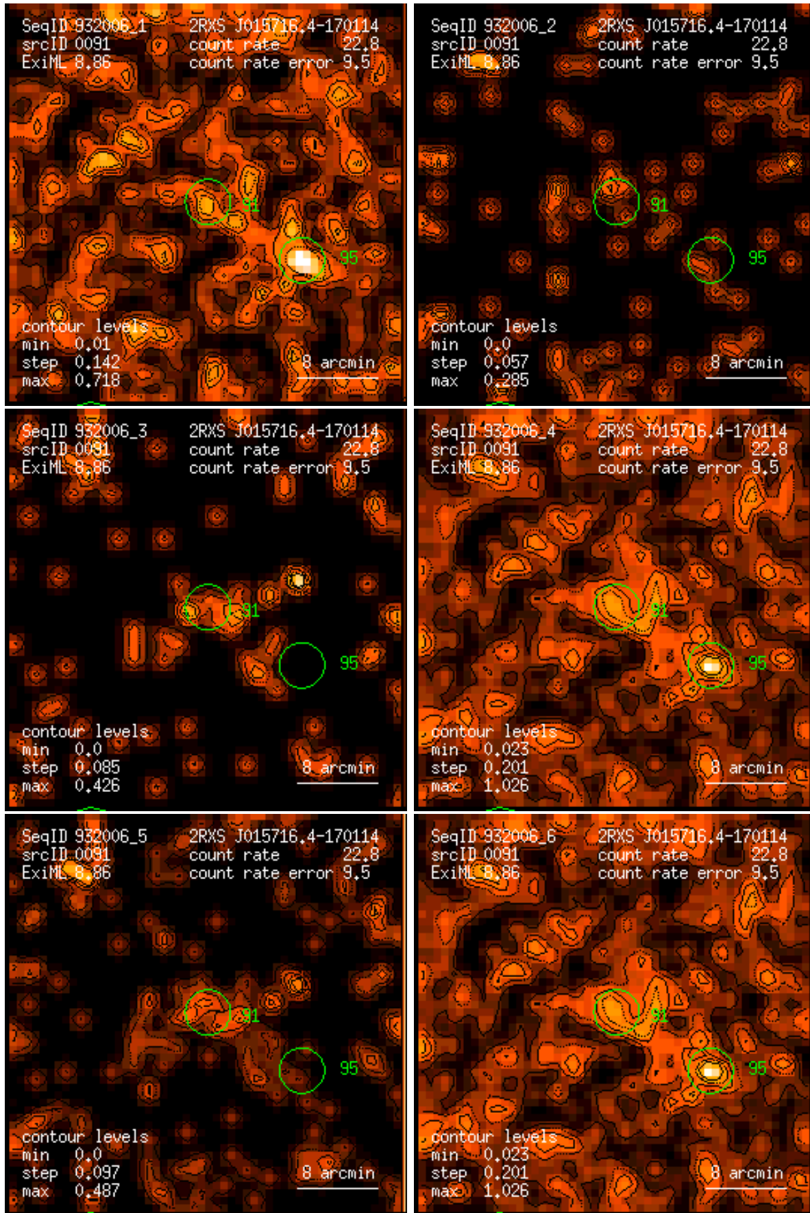
Figure 91: RASS 932006: detection 0091: band rate images, Gaussian filter: (1) PSPC channels 11 – 41, (2) 52 – 90, (3) 91 – 201, (4) 11 – 235, (5) 52 – 201, (6) 11 – 201. Broad band rates in counts/ks. Band rate contour levels in counts/ks/arcmin 2 .
