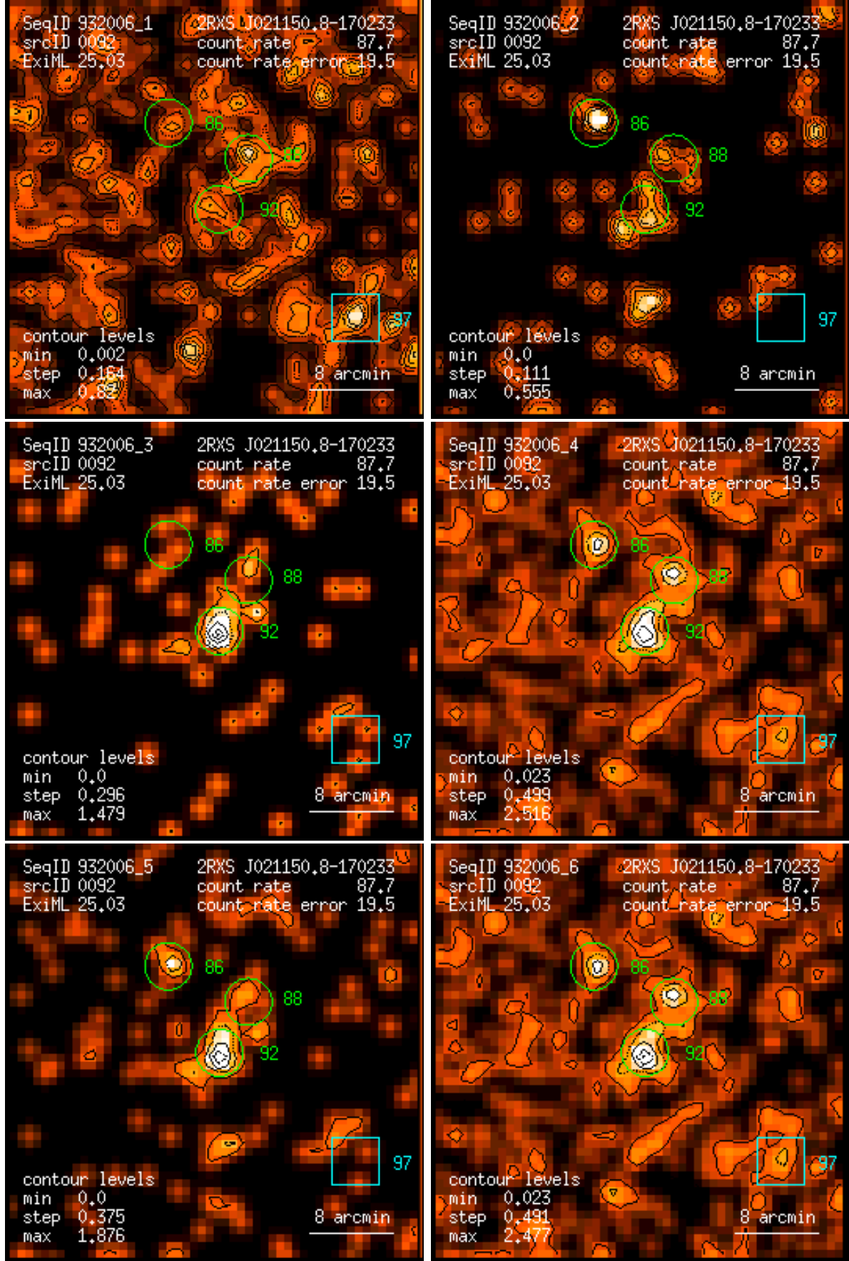
Figure 92: RASS 932006: detection 0092: band rate images, Gaussian filter: (1) PSPC channels 11 – 41, (2) 52 – 90, (3) 91 – 201, (4) 11 – 235, (5) 52 – 201, (6) 11 – 201. Broad band rates in counts/ks. Band rate contour levels in counts/ks/arcmin 2 .
