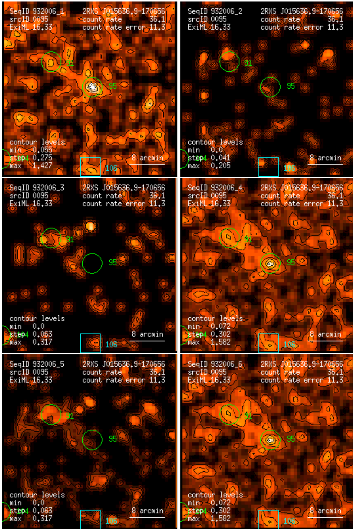
Figure 95: RASS 932006: detection 0095: band rate images, Gaussian filter: (1) PSPC channels 11 – 41, (2) 52 – 90, (3) 91 – 201, (4) 11 – 235, (5) 52 – 201, (6) 11 – 201. Broad band rates in counts/ks. Band rate contour levels in counts/ks/arcmin 2 .
