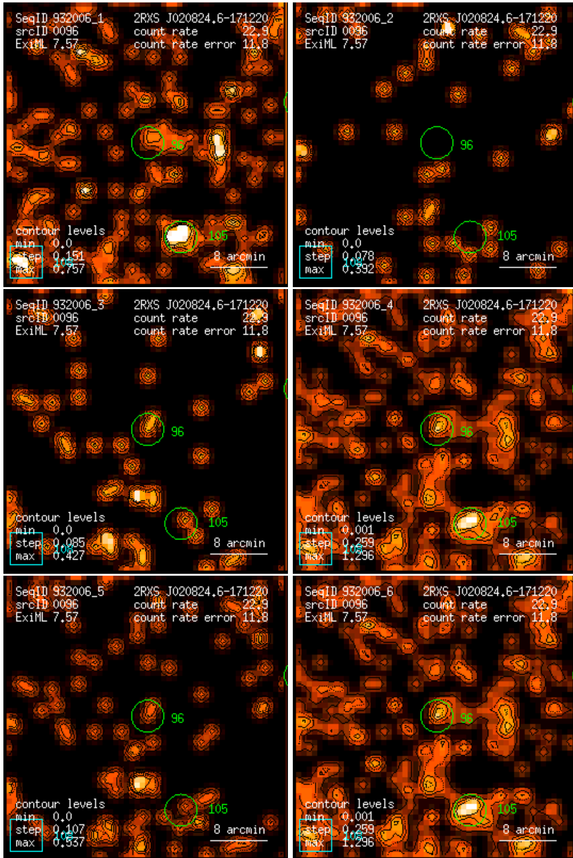
Figure 96: RASS 932006: detection 0096: band rate images, Gaussian filter: (1) PSPC channels 11 – 41, (2) 52 – 90, (3) 91 – 201, (4) 11 – 235, (5) 52 – 201, (6) 11 – 201. Broad band rates in counts/ks. Band rate contour levels in counts/ks/arcmin 2 .
