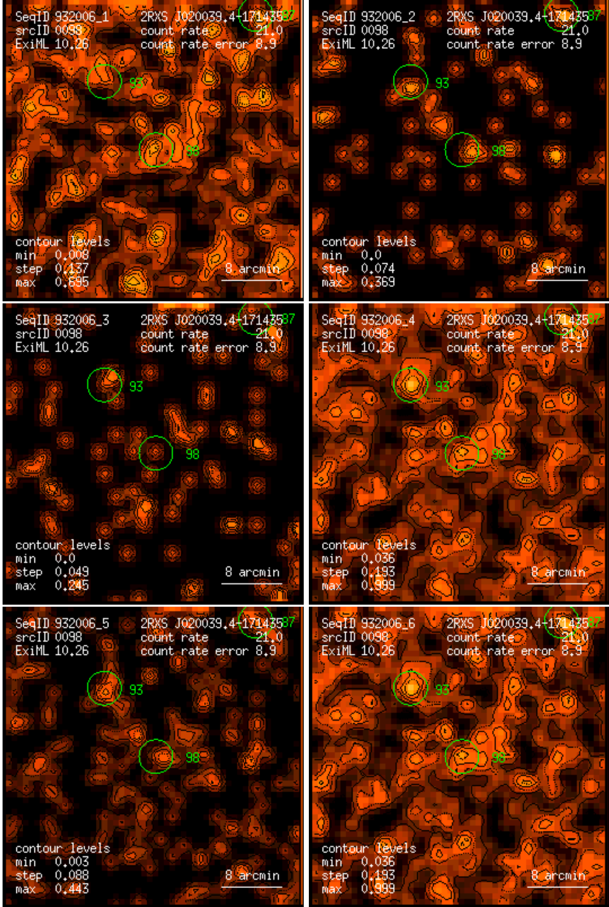
Figure 98: RASS 932006: detection 0098: band rate images, Gaussian filter: (1) PSPC channels 11 – 41, (2) 52 – 90, (3) 91 – 201, (4) 11 – 235, (5) 52 – 201, (6) 11 – 201. Broad band rates in counts/ks. Band rate contour levels in counts/ks/arcmin 2 .
