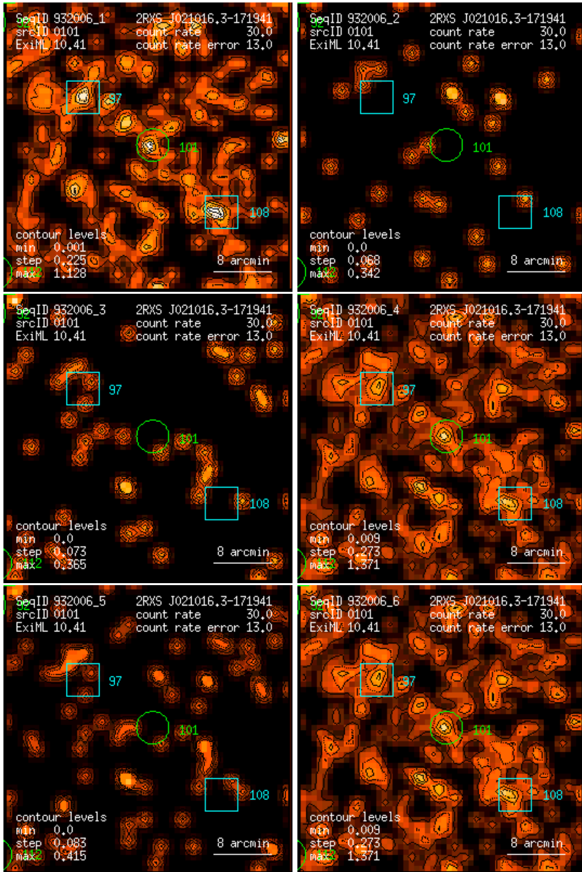
Figure 101: RASS 932006: detection 0101: band rate images, Gaussian filter: (1) PSPC channels 11 – 41, (2) 52 – 90, (3) 91 – 201, (4) 11 – 235, (5) 52 – 201, (6) 11 – 201. Broad band rates in counts/ks. Band rate contour levels in counts/ks/arcmin 2 .
