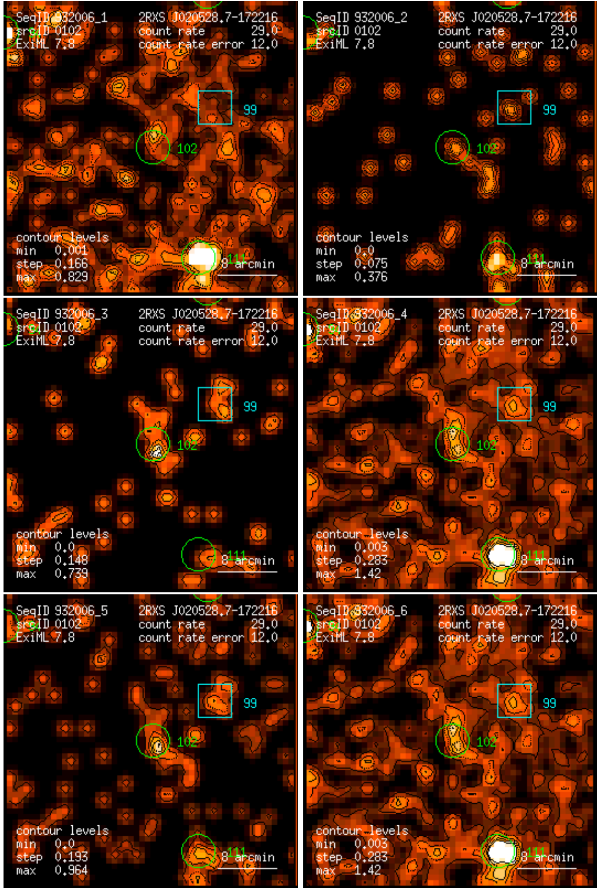
Figure 102: RASS 932006: detection 0102: band rate images, Gaussian filter: (1) PSPC channels 11 – 41, (2) 52 – 90, (3) 91 – 201, (4) 11 – 235, (5) 52 – 201, (6) 11 – 201. Broad band rates in counts/ks. Band rate contour levels in counts/ks/arcmin 2 .
