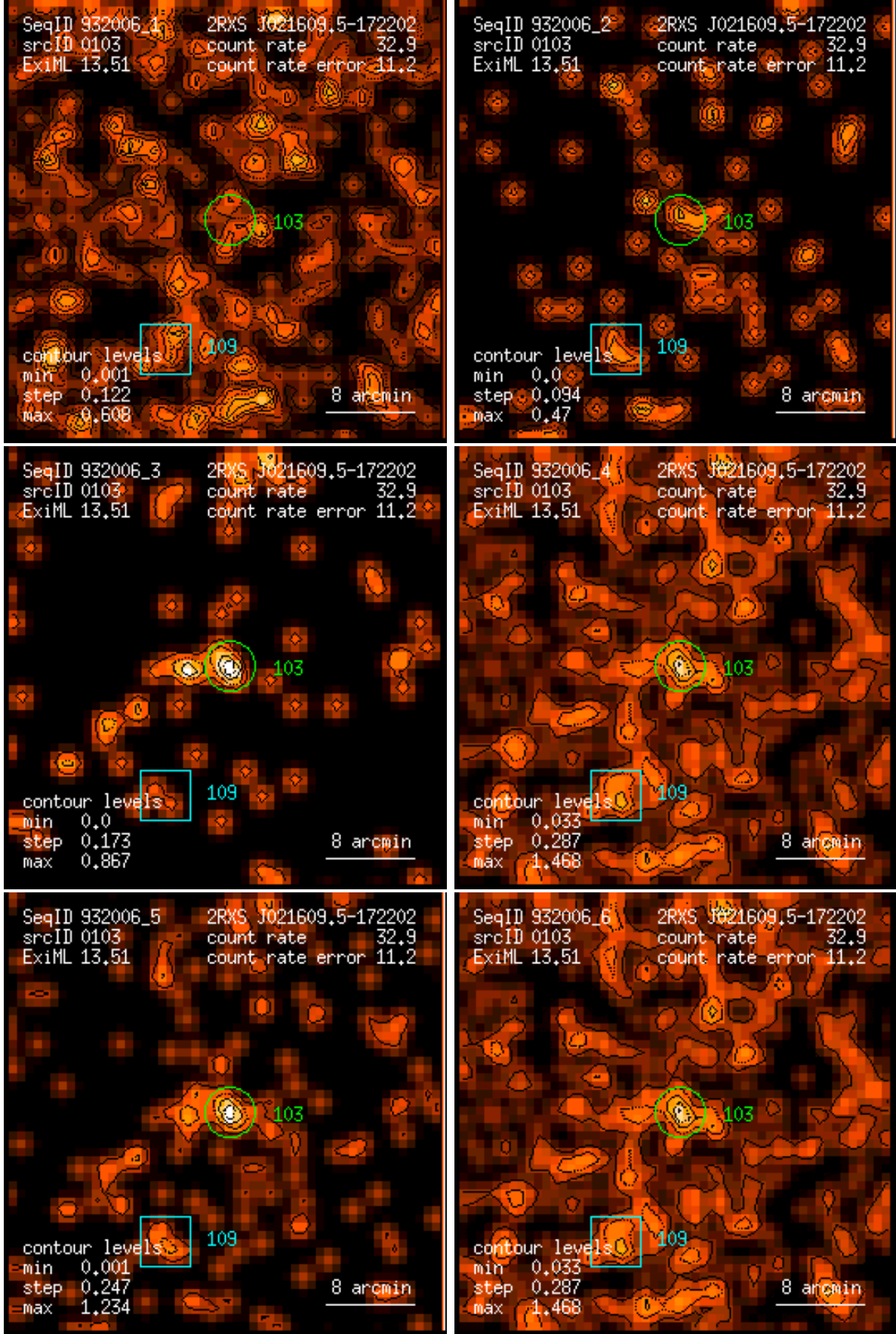
Figure 103: RASS 932006: detection 0103: band rate images, Gaussian filter: (1) PSPC channels 11 – 41, (2) 52 – 90, (3) 91 – 201, (4) 11 – 235, (5) 52 – 201, (6) 11 – 201. Broad band rates in counts/ks. Band rate contour levels in counts/ks/arcmin 2 .
