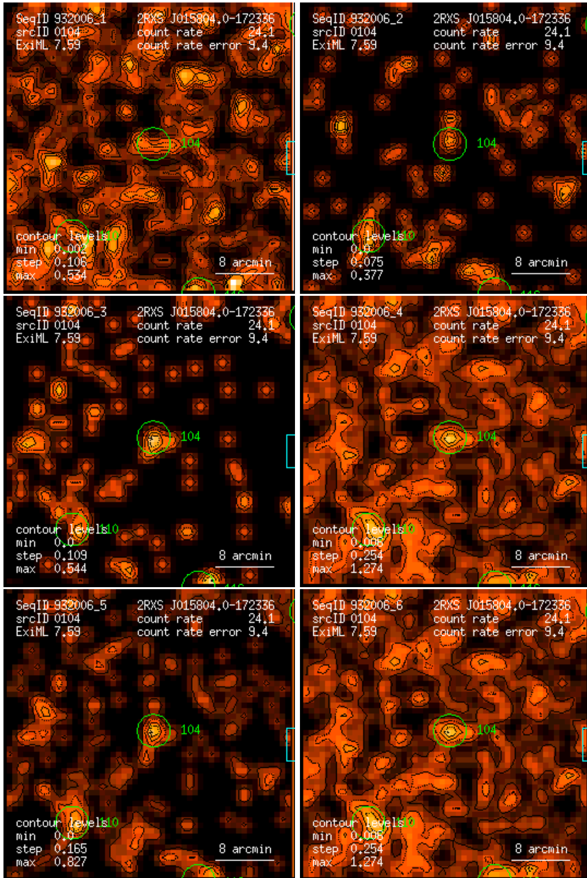
Figure 104: RASS 932006: detection 0104: band rate images, Gaussian filter: (1) PSPC channels 11 – 41, (2) 52 – 90, (3) 91 – 201, (4) 11 – 235, (5) 52 – 201, (6) 11 – 201. Broad band rates in counts/ks. Band rate contour levels in counts/ks/arcmin 2 .
