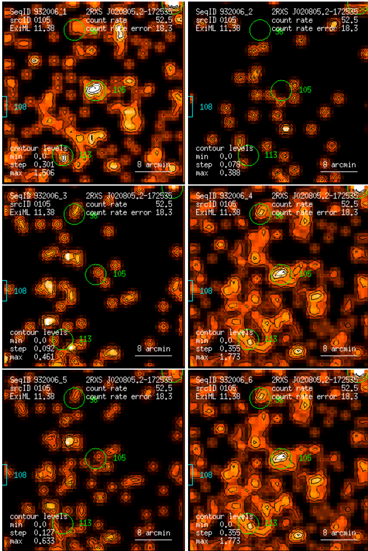
Figure 105: RASS 932006: detection 0105: band rate images, Gaussian filter: (1) PSPC channels 11 – 41, (2) 52 – 90, (3) 91 – 201, (4) 11 – 235, (5) 52 – 201, (6) 11 – 201. Broad band rates in counts/ks. Band rate contour levels in counts/ks/arcmin 2 .
