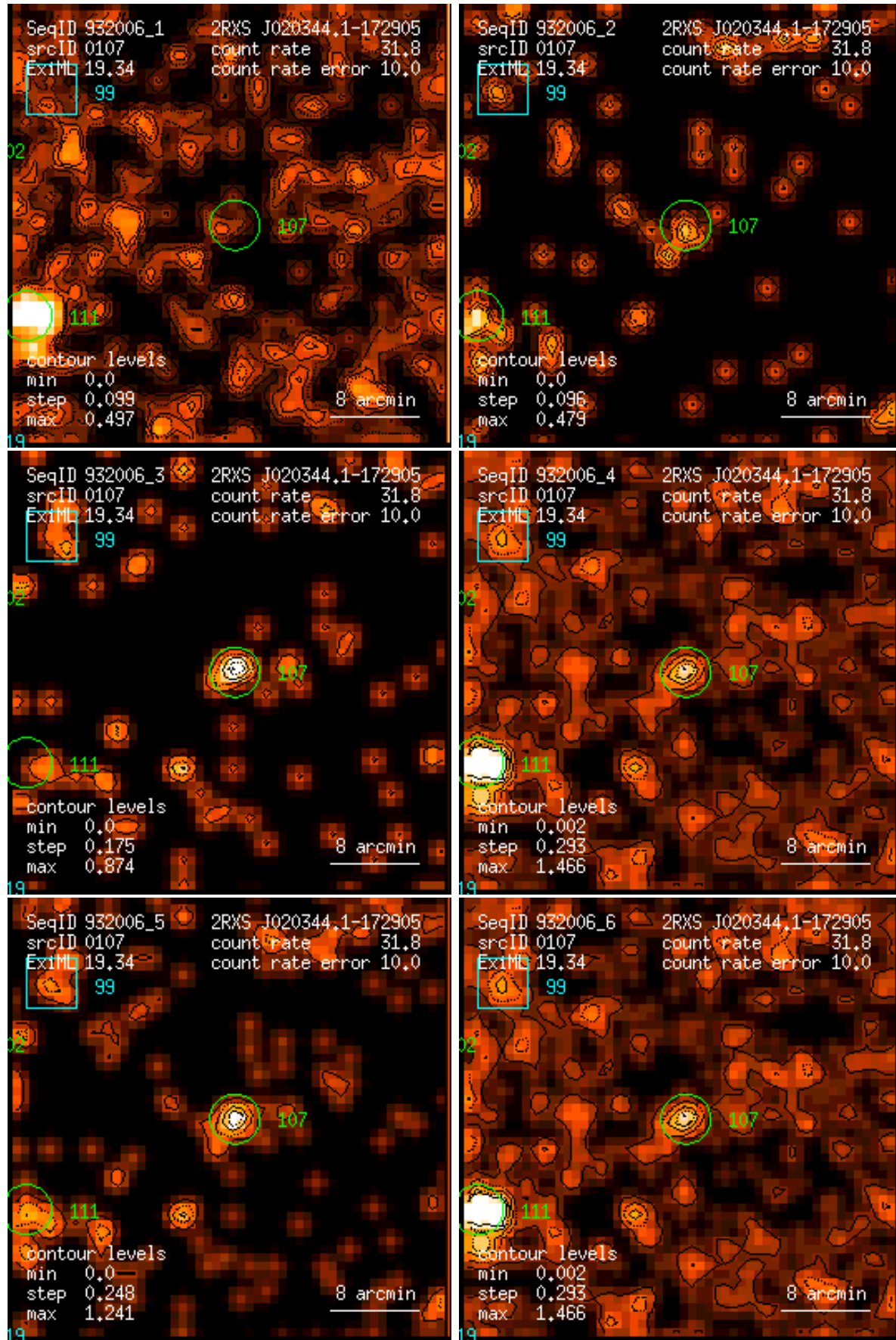
Figure 107: RASS 932006: detection 0107: band rate images, Gaussian filter: (1) PSPC channels 11 – 41, (2) 52 – 90, (3) 91 – 201, (4) 11 – 235, (5) 52 – 201, (6) 11 – 201. Broad band rates in counts/ks. Band rate contour levels in counts/ks/arcmin 2 .
