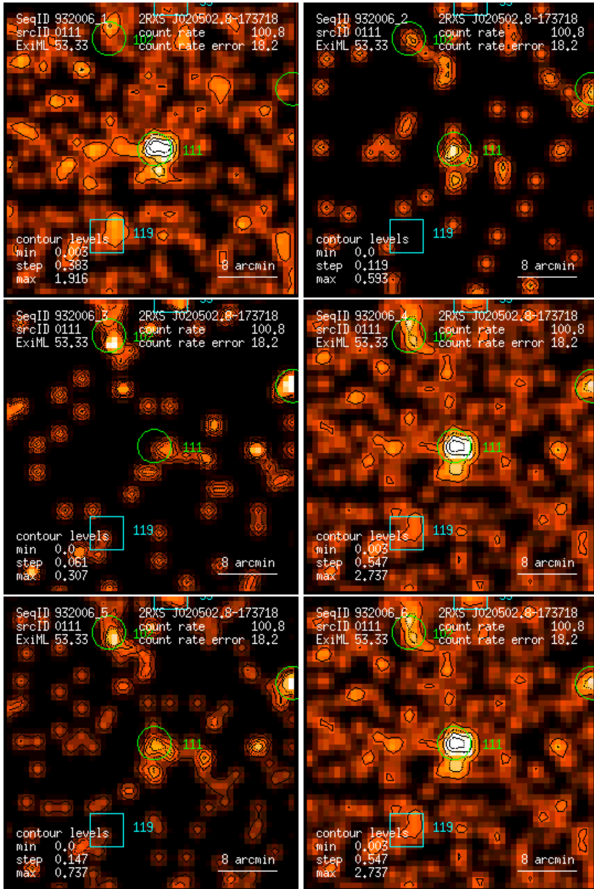
Figure 111: RASS 932006: detection 0111: band rate images, Gaussian filter: (1) PSPC channels 11 – 41, (2) 52 – 90, (3) 91 – 201, (4) 11 – 235, (5) 52 – 201, (6) 11 – 201. Broad band rates in counts/ks. Band rate contour levels in counts/ks/arcmin 2 .
