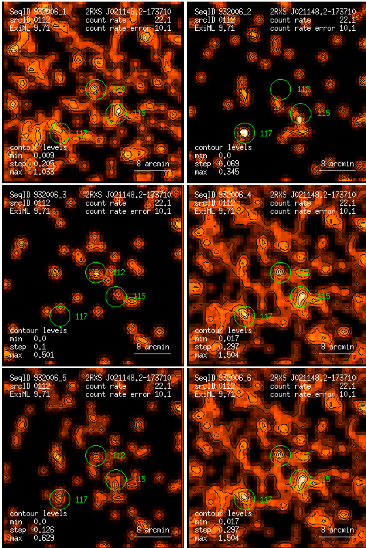
Figure 112: RASS 932006: detection 0112: band rate images, Gaussian filter: (1) PSPC channels 11 – 41, (2) 52 – 90, (3) 91 – 201, (4) 11 – 235, (5) 52 – 201, (6) 11 – 201. Broad band rates in counts/ks. Band rate contour levels in counts/ks/arcmin 2 .
