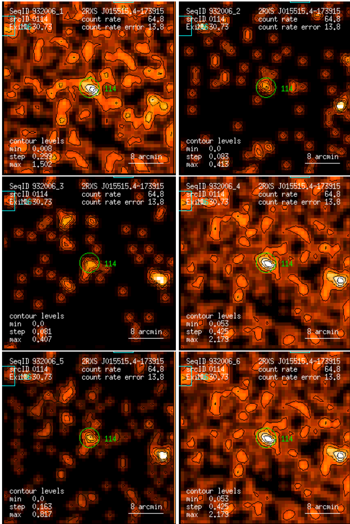
Figure 114: RASS 932006: detection 0114: band rate images, Gaussian filter: (1) PSPC channels 11 – 41, (2) 52 – 90, (3) 91 – 201, (4) 11 – 235, (5) 52 – 201, (6) 11 – 201. Broad band rates in counts/ks. Band rate contour levels in counts/ks/arcmin 2 .
