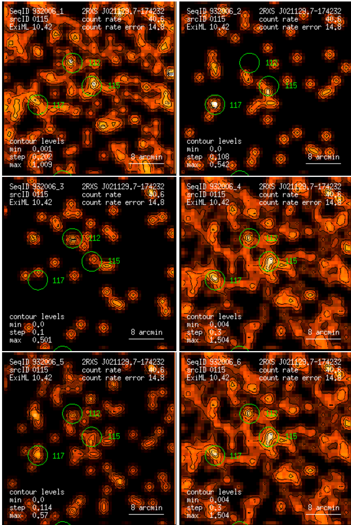
Figure 115: RASS 932006: detection 0115: band rate images, Gaussian filter: (1) PSPC channels 11 – 41, (2) 52 – 90, (3) 91 – 201, (4) 11 – 235, (5) 52 – 201, (6) 11 – 201. Broad band rates in counts/ks. Band rate contour levels in counts/ks/arcmin 2 .
