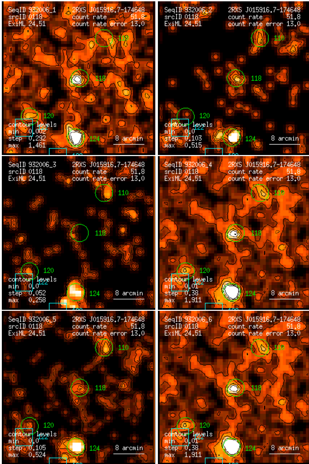
Figure 118: RASS 932006: detection 0118: band rate images, Gaussian filter: (1) PSPC channels 11 – 41, (2) 52 – 90, (3) 91 – 201, (4) 11 – 235, (5) 52 – 201, (6) 11 – 201. Broad band rates in counts/ks. Band rate contour levels in counts/ks/arcmin 2 .
