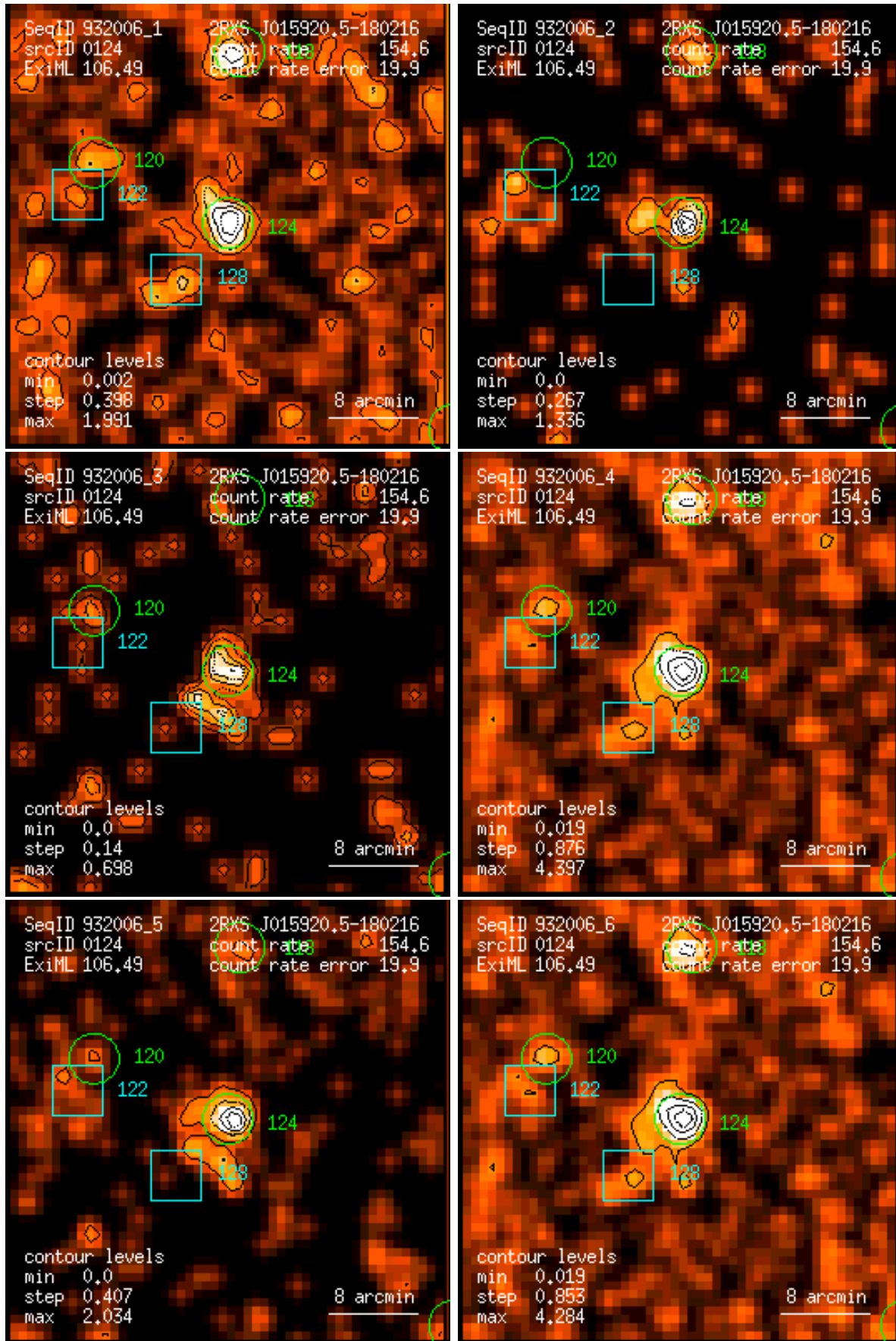
Figure 124: RASS 932006: detection 0124: band rate images, Gaussian filter: (1) PSPC channels 11 – 41, (2) 52 – 90, (3) 91 – 201, (4) 11 – 235, (5) 52 – 201, (6) 11 – 201. Broad band rates in counts/ks. Band rate contour levels in counts/ks/arcmin 2 .
