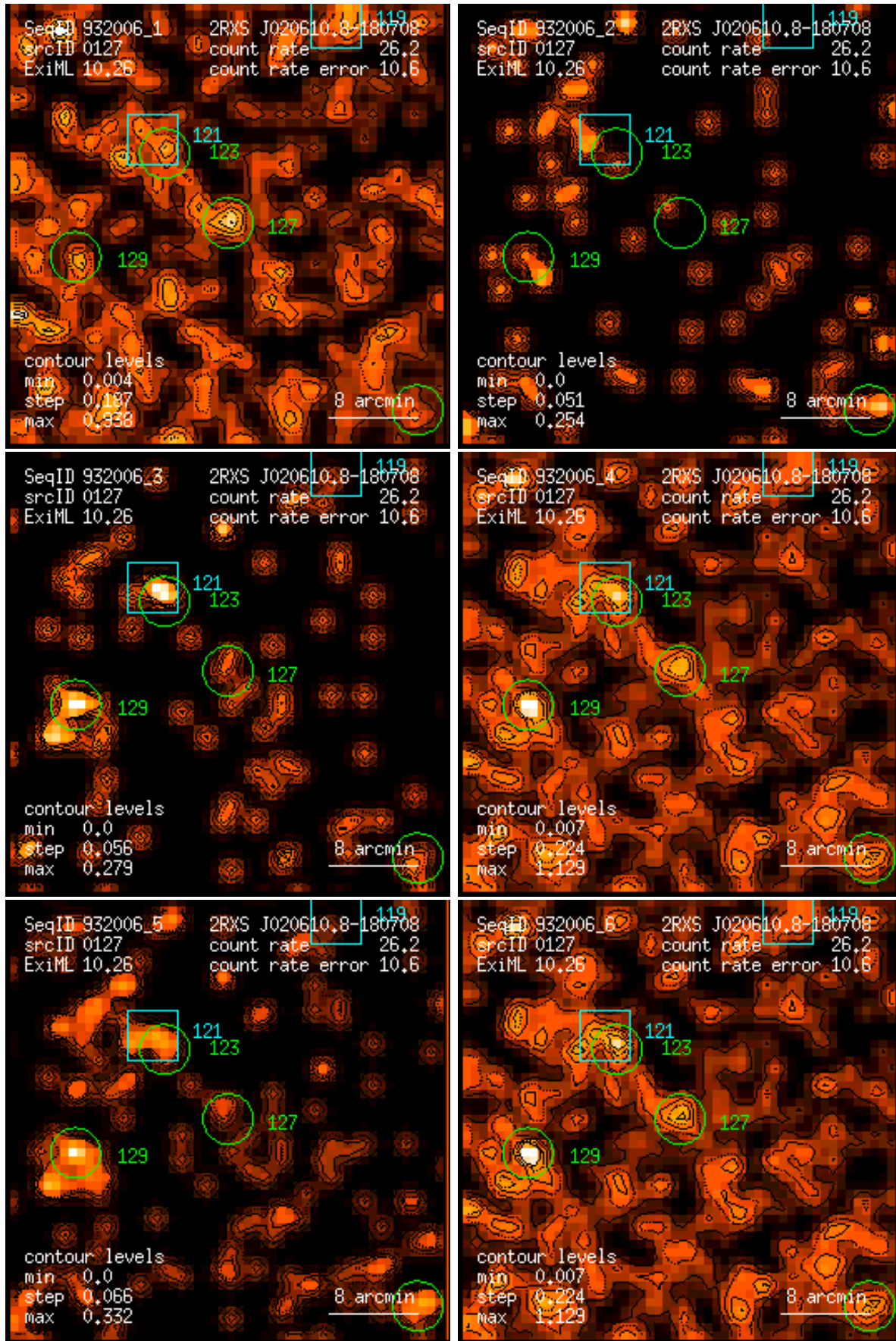
Figure 127: RASS 932006: detection 0127: band rate images, Gaussian filter: (1) PSPC channels 11 – 41, (2) 52 – 90, (3) 91 – 201, (4) 11 – 235, (5) 52 – 201, (6) 11 – 201. Broad band rates in counts/ks. Band rate contour levels in counts/ks/arcmin 2 .
