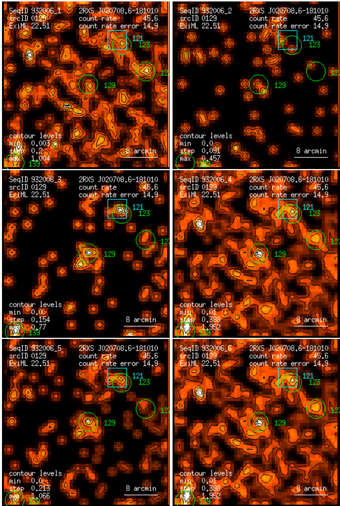
Figure 129: RASS 932006: detection 0129: band rate images, Gaussian filter: (1) PSPC channels 11 – 41, (2) 52 – 90, (3) 91 – 201, (4) 11 – 235, (5) 52 – 201, (6) 11 – 201. Broad band rates in counts/ks. Band rate contour levels in counts/ks/arcmin 2 .
