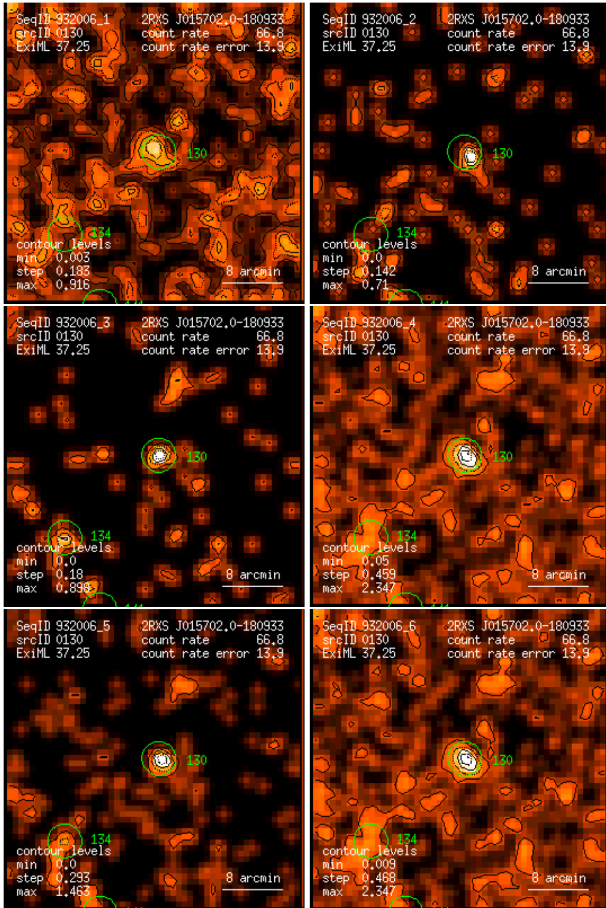
Figure 130: RASS 932006: detection 0130: band rate images, Gaussian filter: (1) PSPC channels 11 – 41, (2) 52 – 90, (3) 91 – 201, (4) 11 – 235, (5) 52 – 201, (6) 11 – 201. Broad band rates in counts/ks. Band rate contour levels in counts/ks/arcmin 2 .
