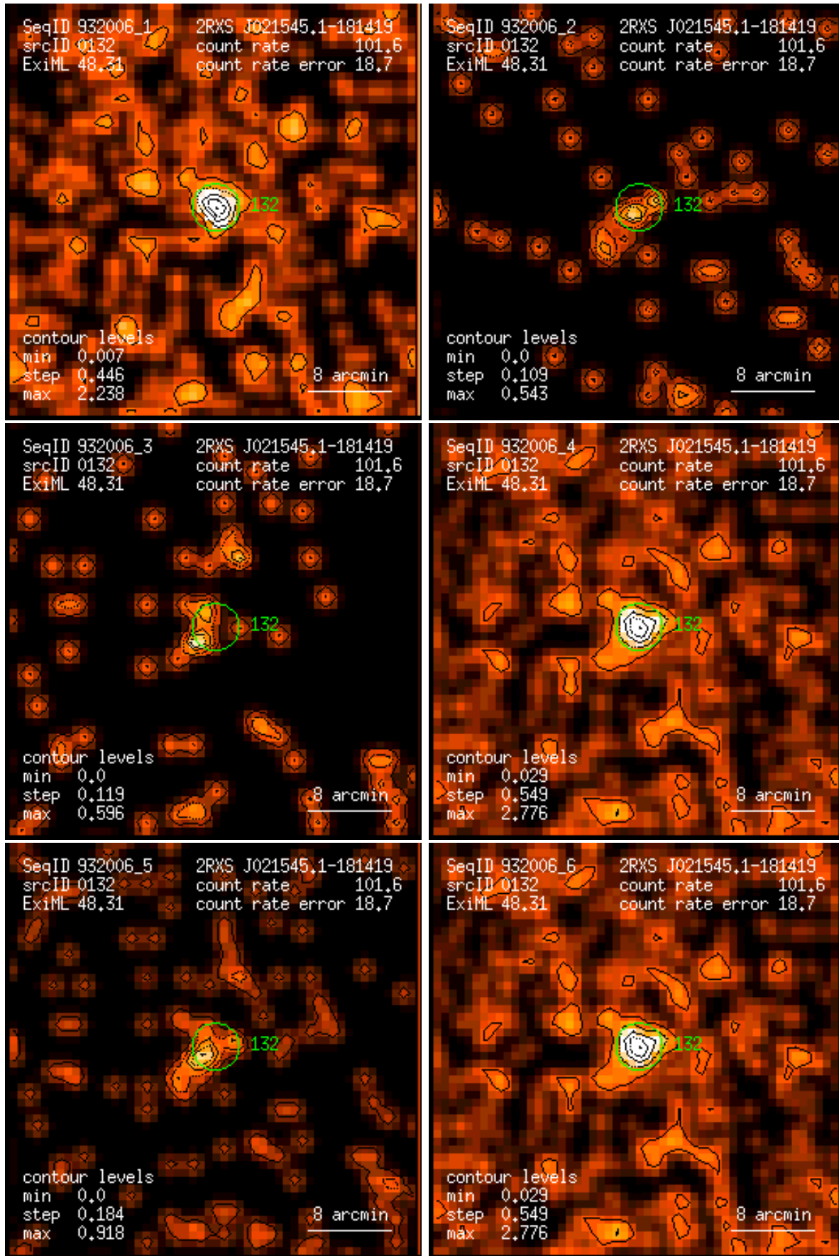
Figure 132: RASS 932006: detection 0132: band rate images, Gaussian filter: (1) PSPC channels 11 – 41, (2) 52 – 90, (3) 91 – 201, (4) 11 – 235, (5) 52 – 201, (6) 11 – 201. Broad band rates in counts/ks. Band rate contour levels in counts/ks/arcmin 2 .
