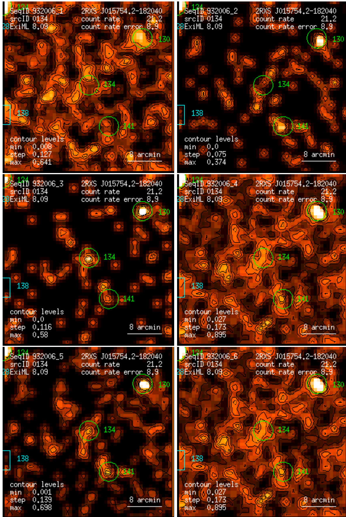
Figure 134: RASS 932006: detection 0134: band rate images, Gaussian filter: (1) PSPC channels 11 – 41, (2) 52 – 90, (3) 91 – 201, (4) 11 – 235, (5) 52 – 201, (6) 11 – 201. Broad band rates in counts/ks. Band rate contour levels in counts/ks/arcmin 2 .
