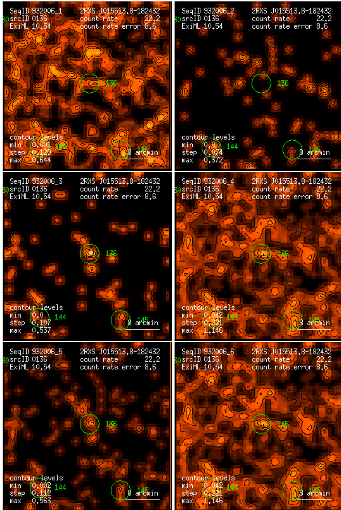
Figure 136: RASS 932006: detection 0136: band rate images, Gaussian filter: (1) PSPC channels 11 – 41, (2) 52 – 90, (3) 91 – 201, (4) 11 – 235, (5) 52 – 201, (6) 11 – 201. Broad band rates in counts/ks. Band rate contour levels in counts/ks/arcmin 2 .
