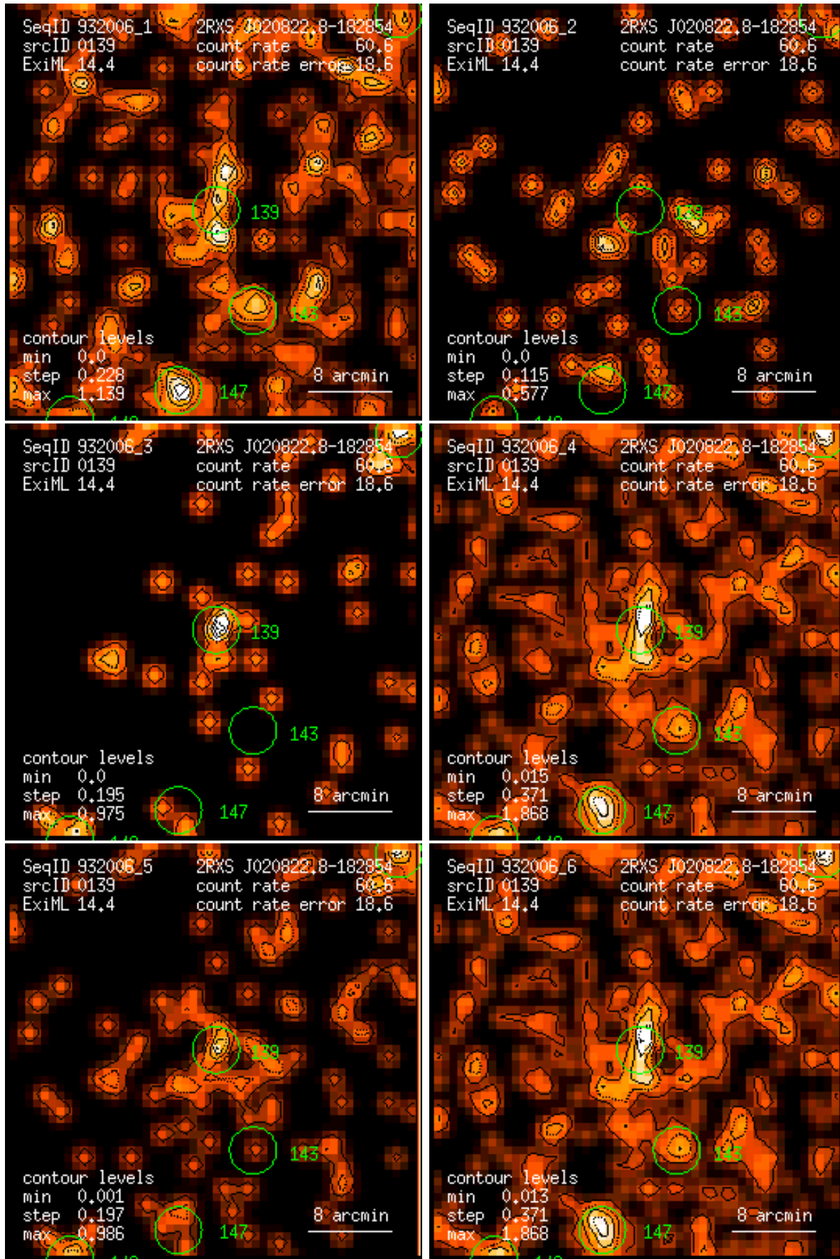
Figure 139: RASS 932006: detection 0139: band rate images, Gaussian filter: (1) PSPC channels 11 – 41, (2) 52 – 90, (3) 91 – 201, (4) 11 – 235, (5) 52 – 201, (6) 11 – 201. Broad band rates in counts/ks. Band rate contour levels in counts/ks/arcmin 2 .
