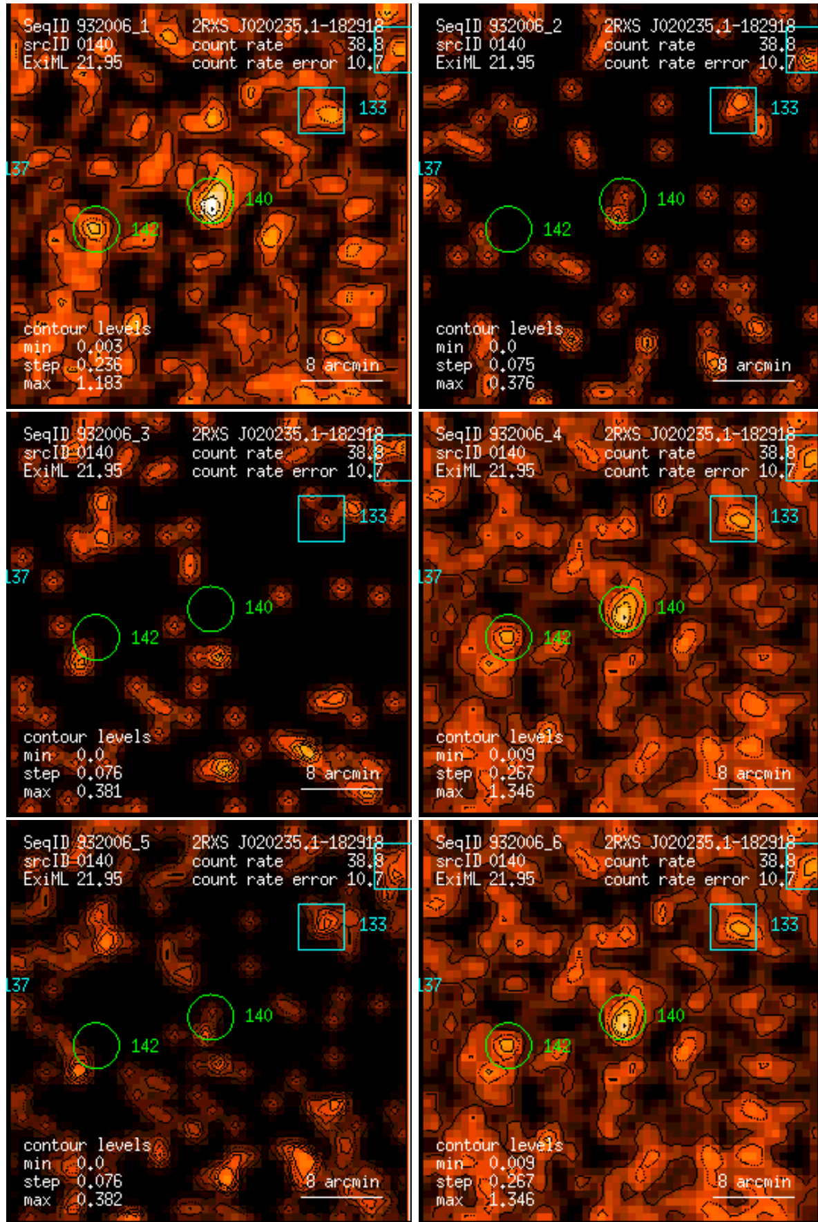
Figure 140: RASS 932006: detection 0140: band rate images, Gaussian filter: (1) PSPC channels 11 – 41, (2) 52 – 90, (3) 91 – 201, (4) 11 – 235, (5) 52 – 201, (6) 11 – 201. Broad band rates in counts/ks. Band rate contour levels in counts/ks/arcmin 2 .
