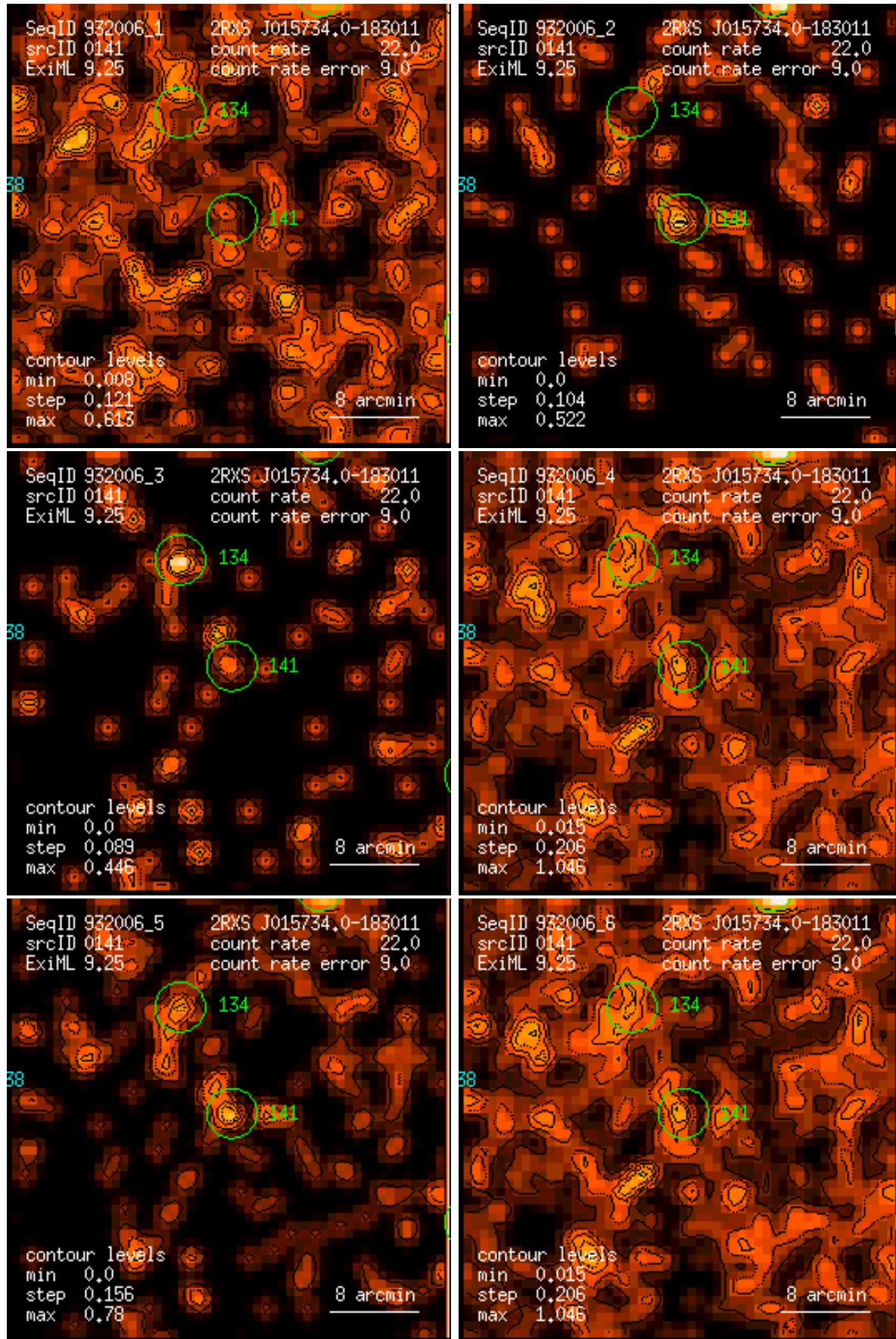
Figure 141: RASS 932006: detection 0141: band rate images, Gaussian filter: (1) PSPC channels 11 – 41, (2) 52 – 90, (3) 91 – 201, (4) 11 – 235, (5) 52 – 201, (6) 11 – 201. Broad band rates in counts/ks. Band rate contour levels in counts/ks/arcmin 2 .
