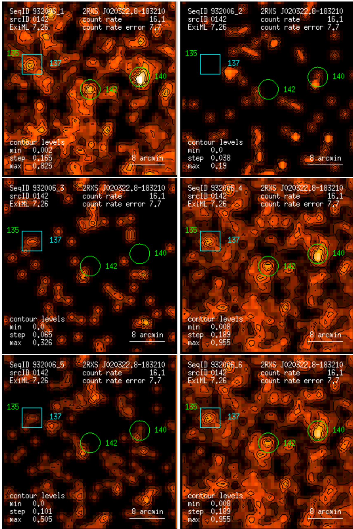
Figure 142: RASS 932006: detection 0142: band rate images, Gaussian filter: (1) PSPC channels 11 – 41, (2) 52 – 90, (3) 91 – 201, (4) 11 – 235, (5) 52 – 201, (6) 11 – 201. Broad band rates in counts/ks. Band rate contour levels in counts/ks/arcmin 2 .
