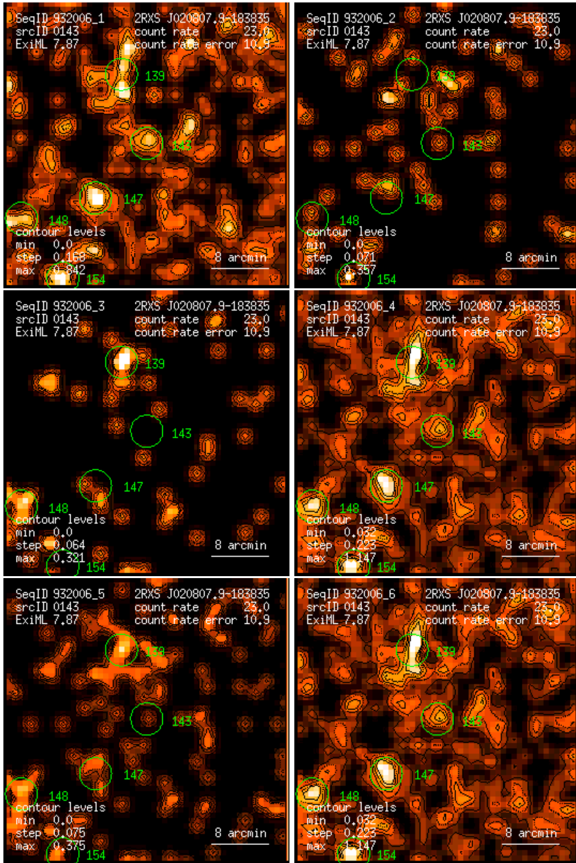
Figure 143: RASS 932006: detection 0143: band rate images, Gaussian filter: (1) PSPC channels 11 – 41, (2) 52 – 90, (3) 91 – 201, (4) 11 – 235, (5) 52 – 201, (6) 11 – 201. Broad band rates in counts/ks. Band rate contour levels in counts/ks/arcmin 2 .
