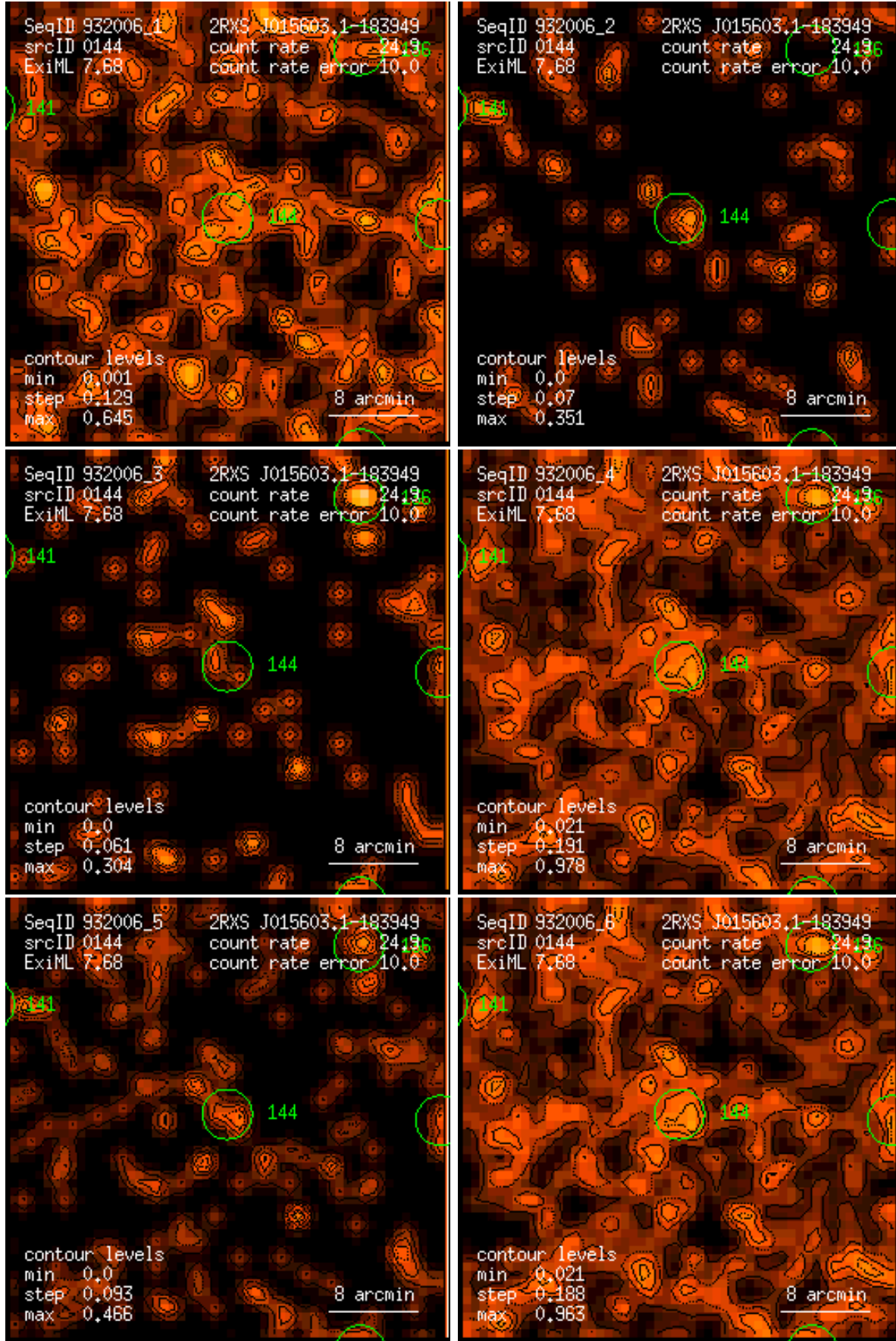
Figure 144: RASS 932006: detection 0144: band rate images, Gaussian filter: (1) PSPC channels 11 – 41, (2) 52 – 90, (3) 91 – 201, (4) 11 – 235, (5) 52 – 201, (6) 11 – 201. Broad band rates in counts/ks. Band rate contour levels in counts/ks/arcmin 2 .
