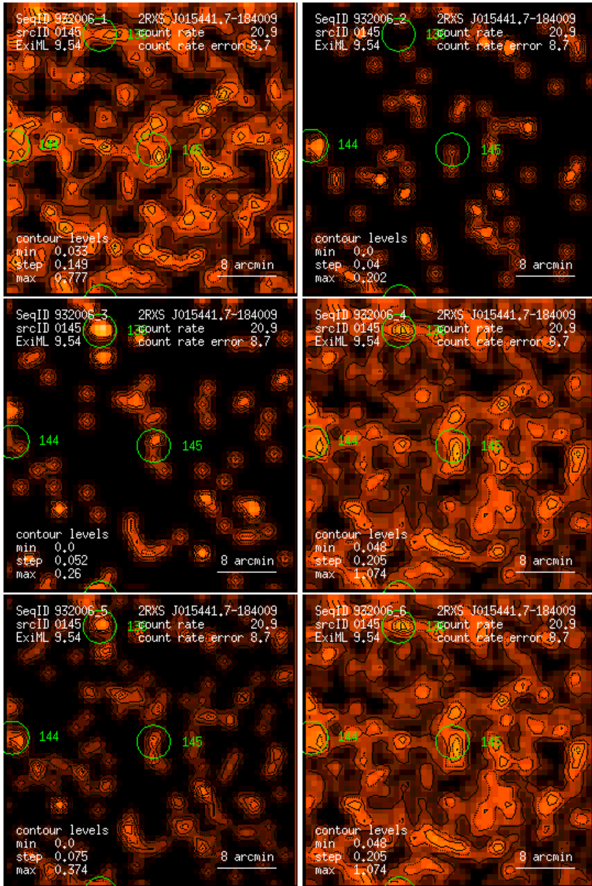
Figure 145: RASS 932006: detection 0145: band rate images, Gaussian filter: (1) PSPC channels 11 – 41, (2) 52 – 90, (3) 91 – 201, (4) 11 – 235, (5) 52 – 201, (6) 11 – 201. Broad band rates in counts/ks. Band rate contour levels in counts/ks/arcmin 2 .
