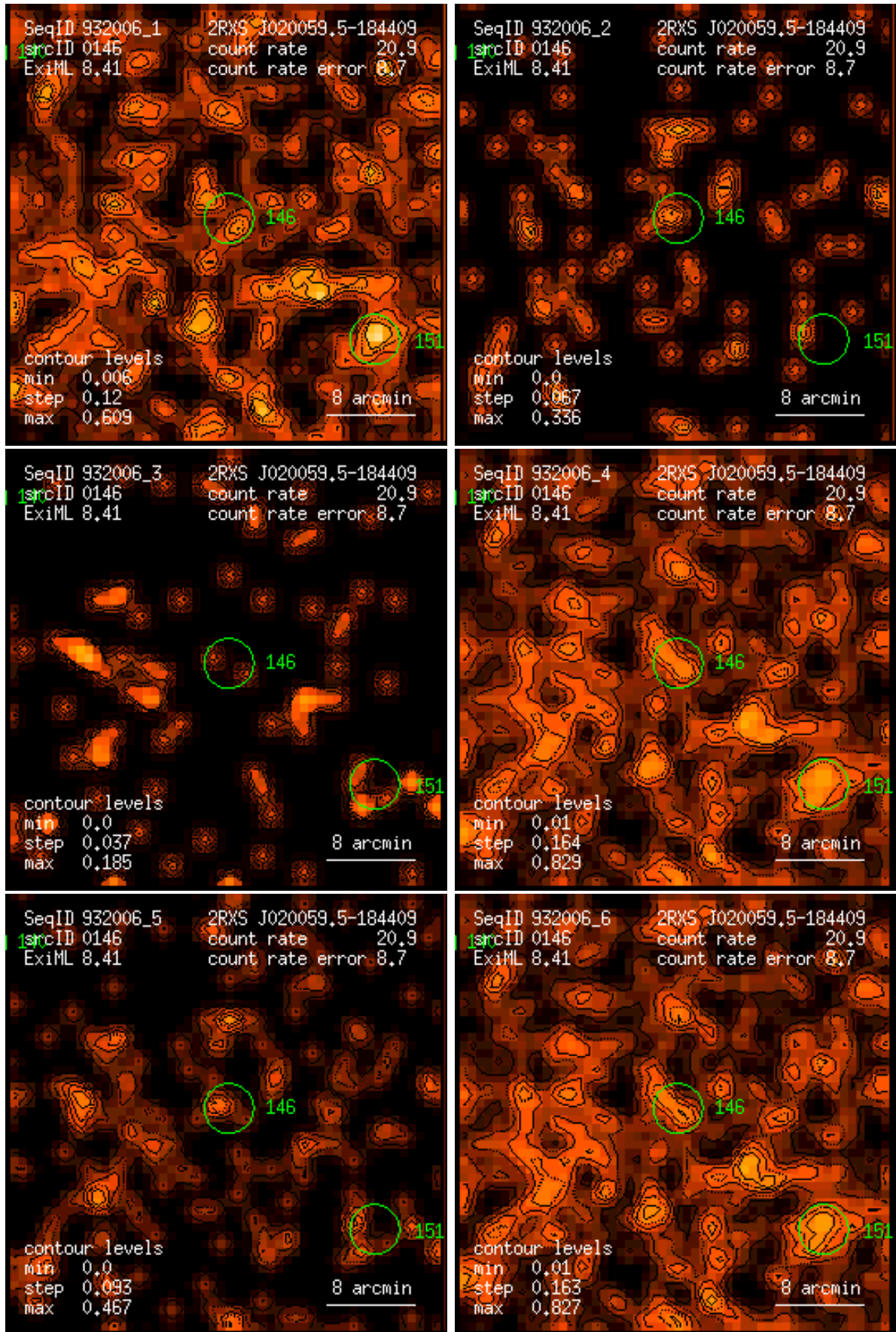
Figure 146: RASS 932006: detection 0146: band rate images, Gaussian filter: (1) PSPC channels 11 – 41, (2) 52 – 90, (3) 91 – 201, (4) 11 – 235, (5) 52 – 201, (6) 11 – 201. Broad band rates in counts/ks. Band rate contour levels in counts/ks/arcmin 2 .
