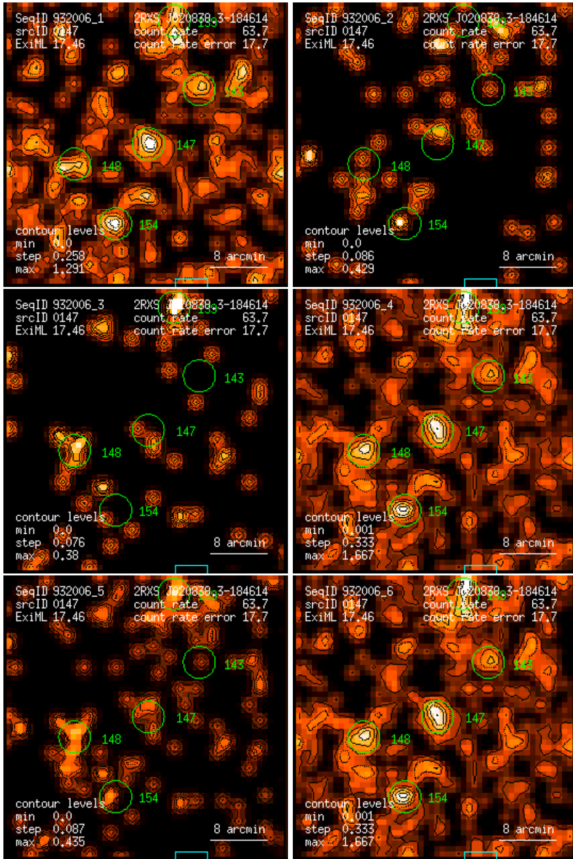
Figure 147: RASS 932006: detection 0147: band rate images, Gaussian filter: (1) PSPC channels 11 – 41, (2) 52 – 90, (3) 91 – 201, (4) 11 – 235, (5) 52 – 201, (6) 11 – 201. Broad band rates in counts/ks. Band rate contour levels in counts/ks/arcmin 2 .
