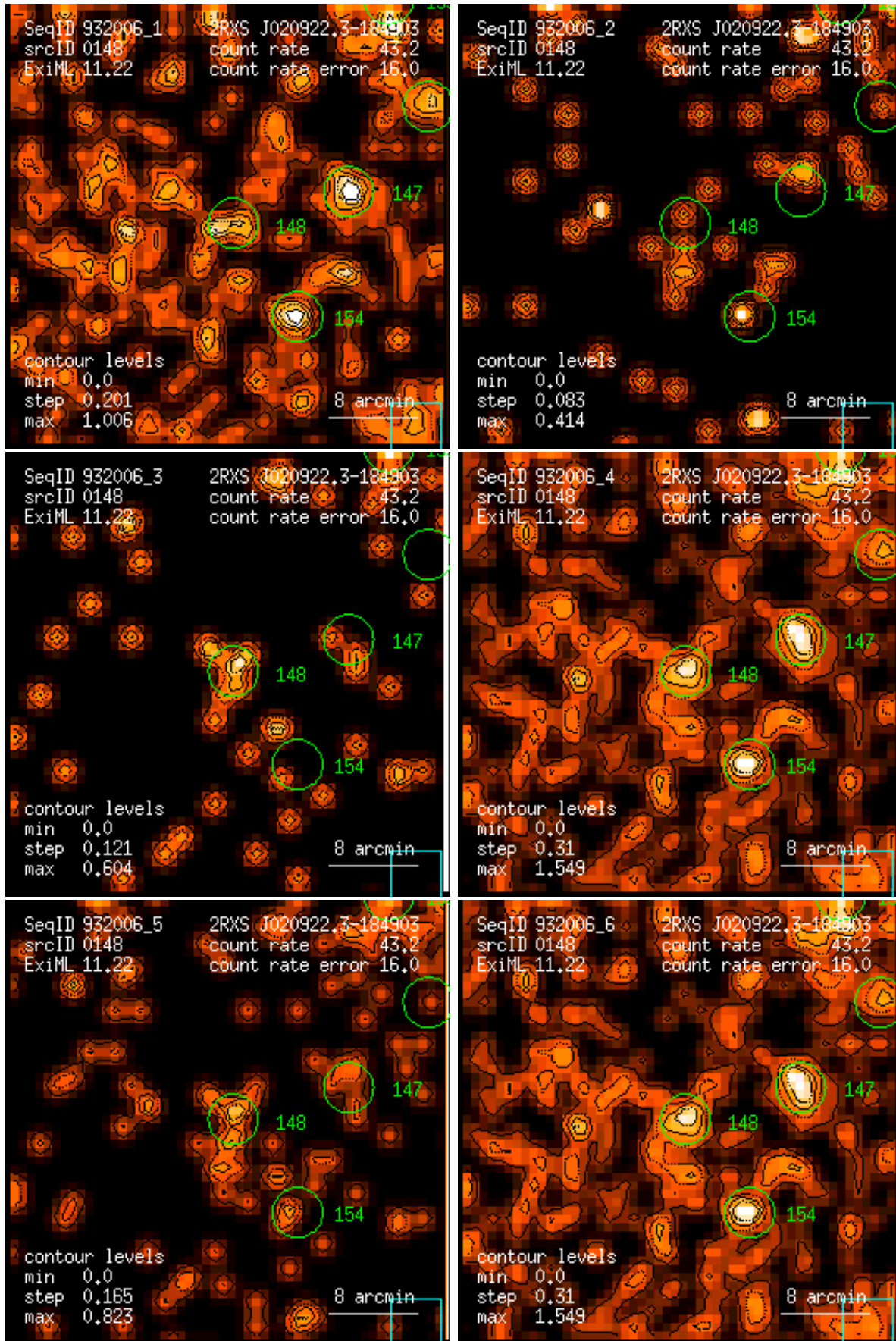
Figure 148: RASS 932006: detection 0148: band rate images, Gaussian filter: (1) PSPC channels 11 – 41, (2) 52 – 90, (3) 91 – 201, (4) 11 – 235, (5) 52 – 201, (6) 11 – 201. Broad band rates in counts/ks. Band rate contour levels in counts/ks/arcmin 2 .
