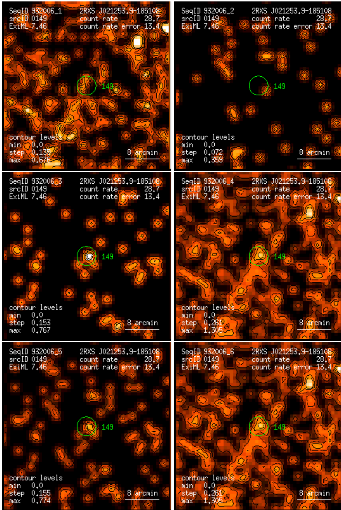
Figure 149: RASS 932006: detection 0149: band rate images, Gaussian filter: (1) PSPC channels 11 – 41, (2) 52 – 90, (3) 91 – 201, (4) 11 – 235, (5) 52 – 201, (6) 11 – 201. Broad band rates in counts/ks. Band rate contour levels in counts/ks/arcmin 2 .
