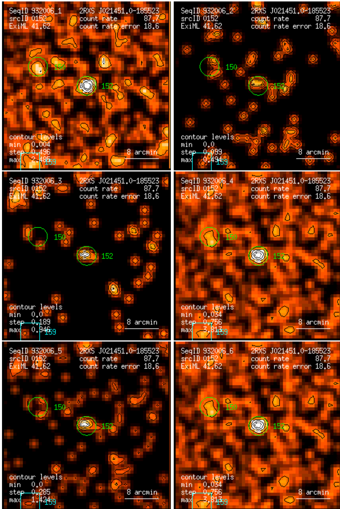
Figure 152: RASS 932006: detection 0152: band rate images, Gaussian filter: (1) PSPC channels 11 – 41, (2) 52 – 90, (3) 91 – 201, (4) 11 – 235, (5) 52 – 201, (6) 11 – 201. Broad band rates in counts/ks. Band rate contour levels in counts/ks/arcmin 2 .
