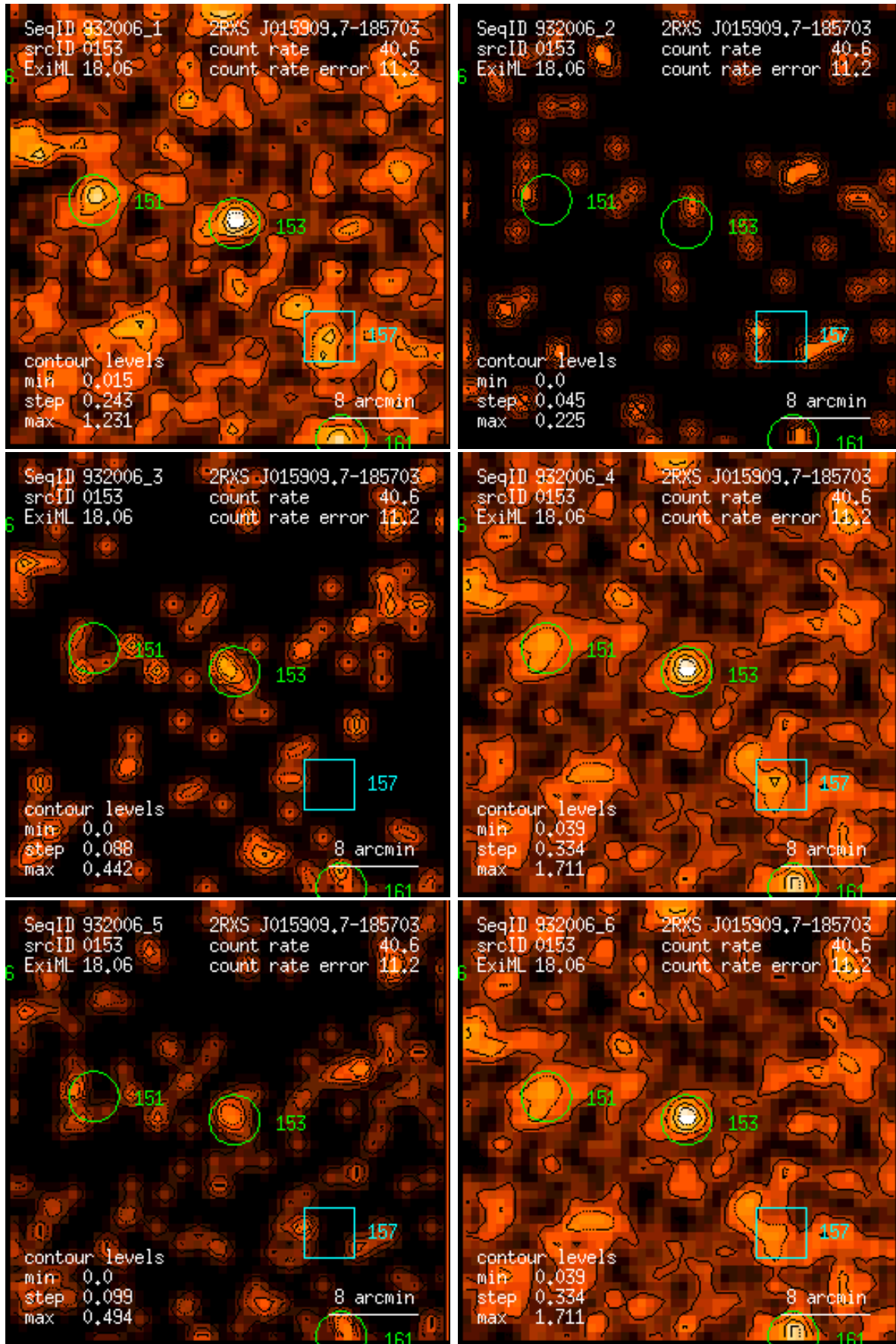
Figure 153: RASS 932006: detection 0153: band rate images, Gaussian filter: (1) PSPC channels 11 – 41, (2) 52 – 90, (3) 91 – 201, (4) 11 – 235, (5) 52 – 201, (6) 11 – 201. Broad band rates in counts/ks. Band rate contour levels in counts/ks/arcmin 2 .
