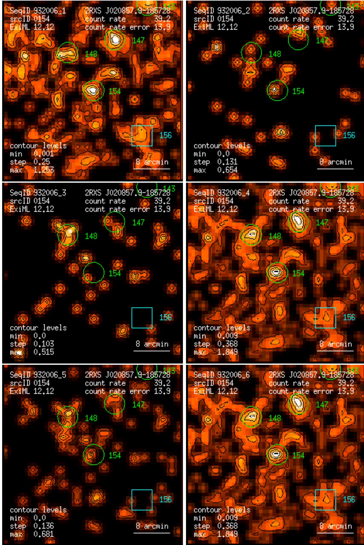
Figure 154: RASS 932006: detection 0154: band rate images, Gaussian filter: (1) PSPC channels 11 – 41, (2) 52 – 90, (3) 91 – 201, (4) 11 – 235, (5) 52 – 201, (6) 11 – 201. Broad band rates in counts/ks. Band rate contour levels in counts/ks/arcmin 2 .
