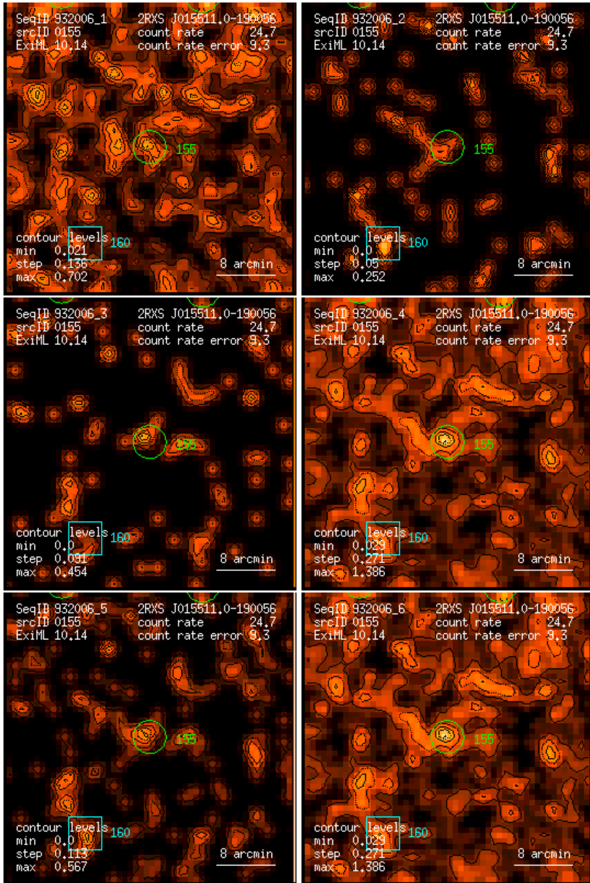
Figure 155: RASS 932006: detection 0155: band rate images, Gaussian filter: (1) PSPC channels 11 – 41, (2) 52 – 90, (3) 91 – 201, (4) 11 – 235, (5) 52 – 201, (6) 11 – 201. Broad band rates in counts/ks. Band rate contour levels in counts/ks/arcmin 2 .
