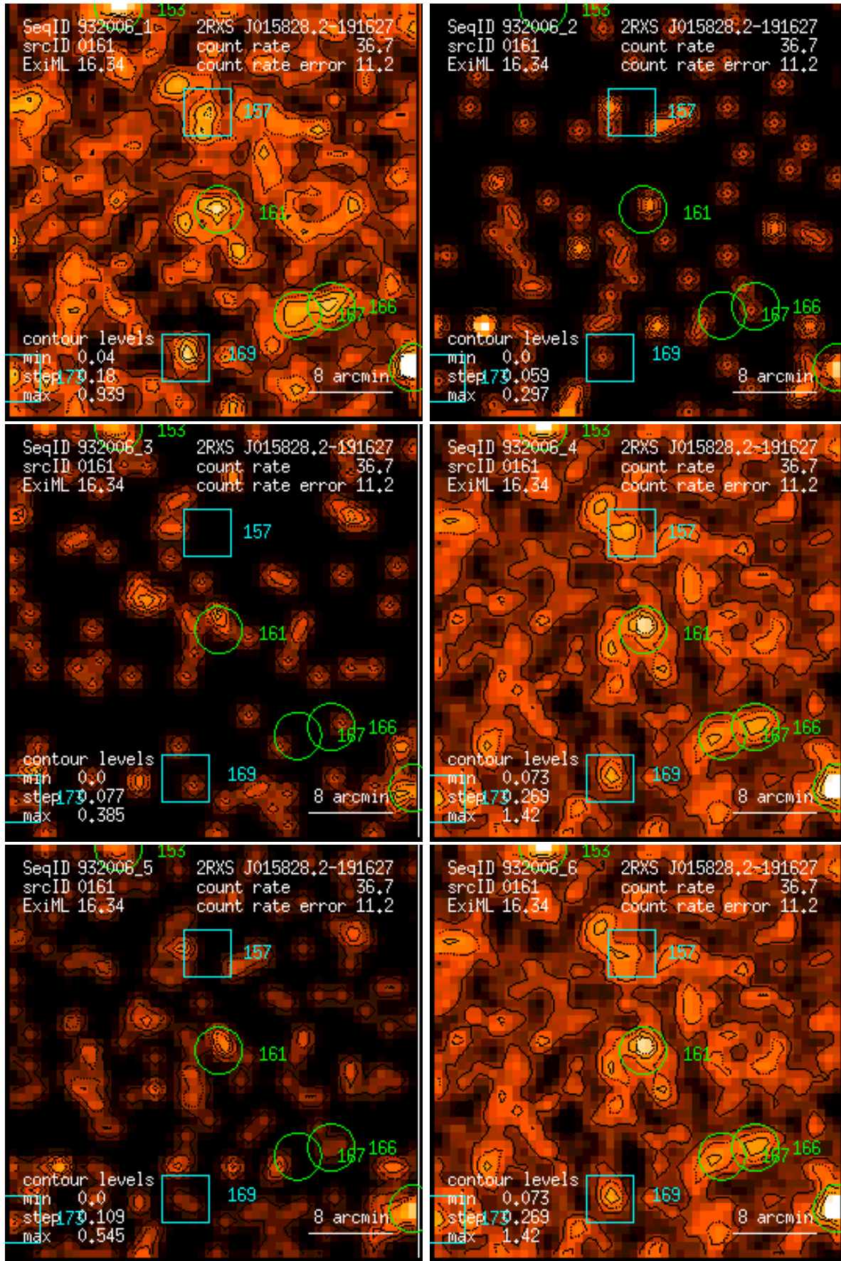
Figure 161: RASS 932006: detection 0161: band rate images, Gaussian filter: (1) PSPC channels 11 – 41, (2) 52 – 90, (3) 91 – 201, (4) 11 – 235, (5) 52 – 201, (6) 11 – 201. Broad band rates in counts/ks. Band rate contour levels in counts/ks/arcmin 2 .
