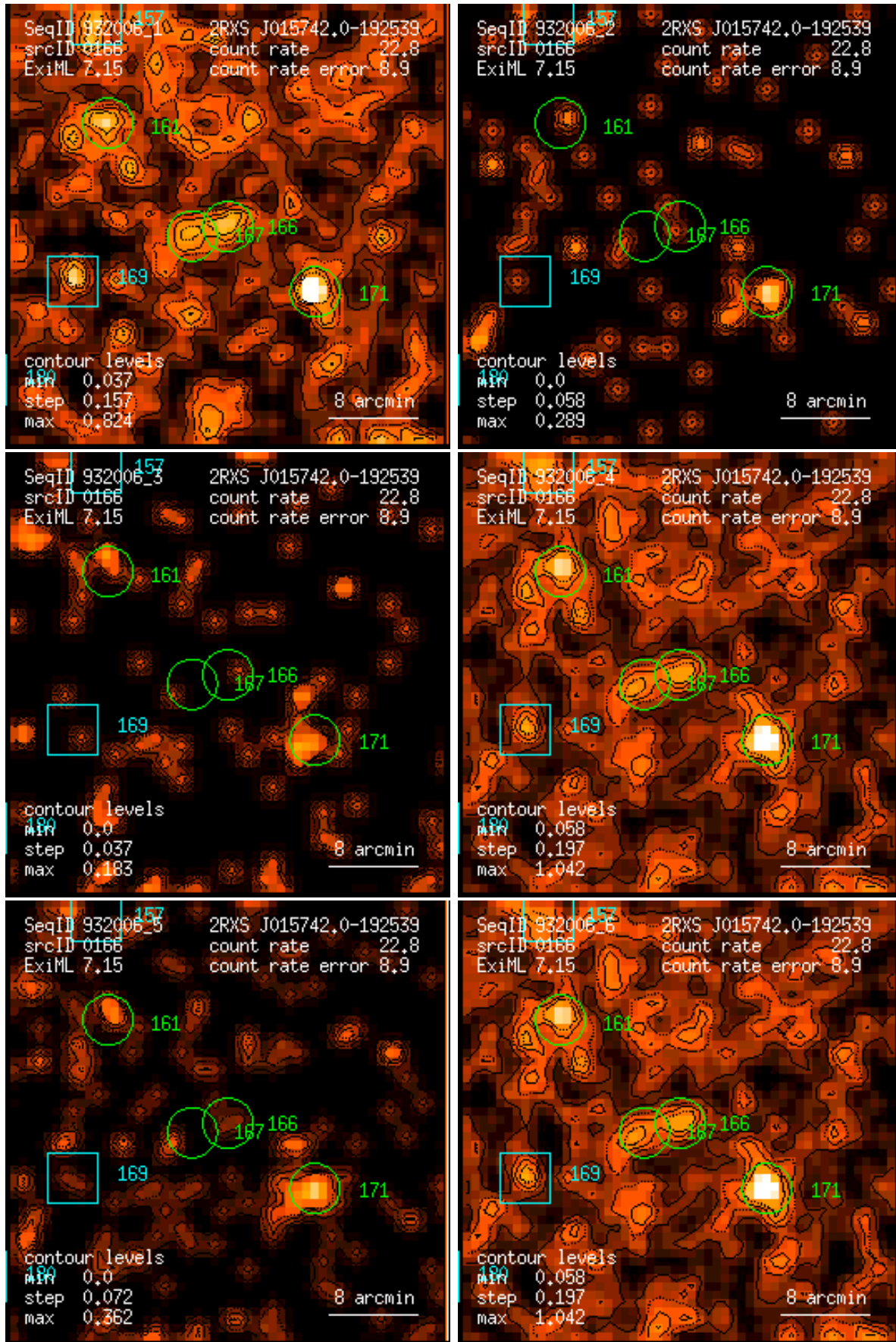
Figure 166: RASS 932006: detection 0166: band rate images, Gaussian filter: (1) PSPC channels 11 – 41, (2) 52 – 90, (3) 91 – 201, (4) 11 – 235, (5) 52 – 201, (6) 11 – 201. Broad band rates in counts/ks. Band rate contour levels in counts/ks/arcmin 2 .
