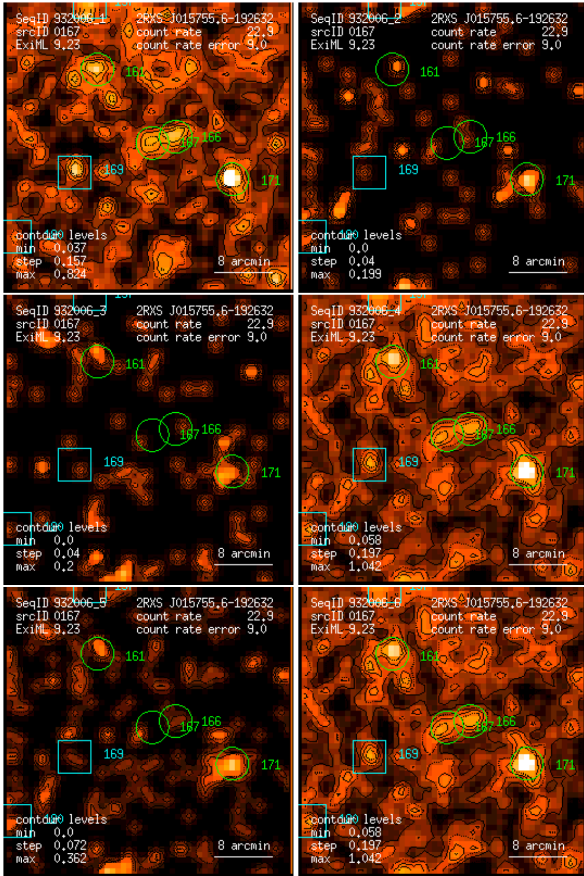
Figure 167: RASS 932006: detection 0167: band rate images, Gaussian filter: (1) PSPC channels 11 – 41, (2) 52 – 90, (3) 91 – 201, (4) 11 – 235, (5) 52 – 201, (6) 11 – 201. Broad band rates in counts/ks. Band rate contour levels in counts/ks/arcmin 2 .
