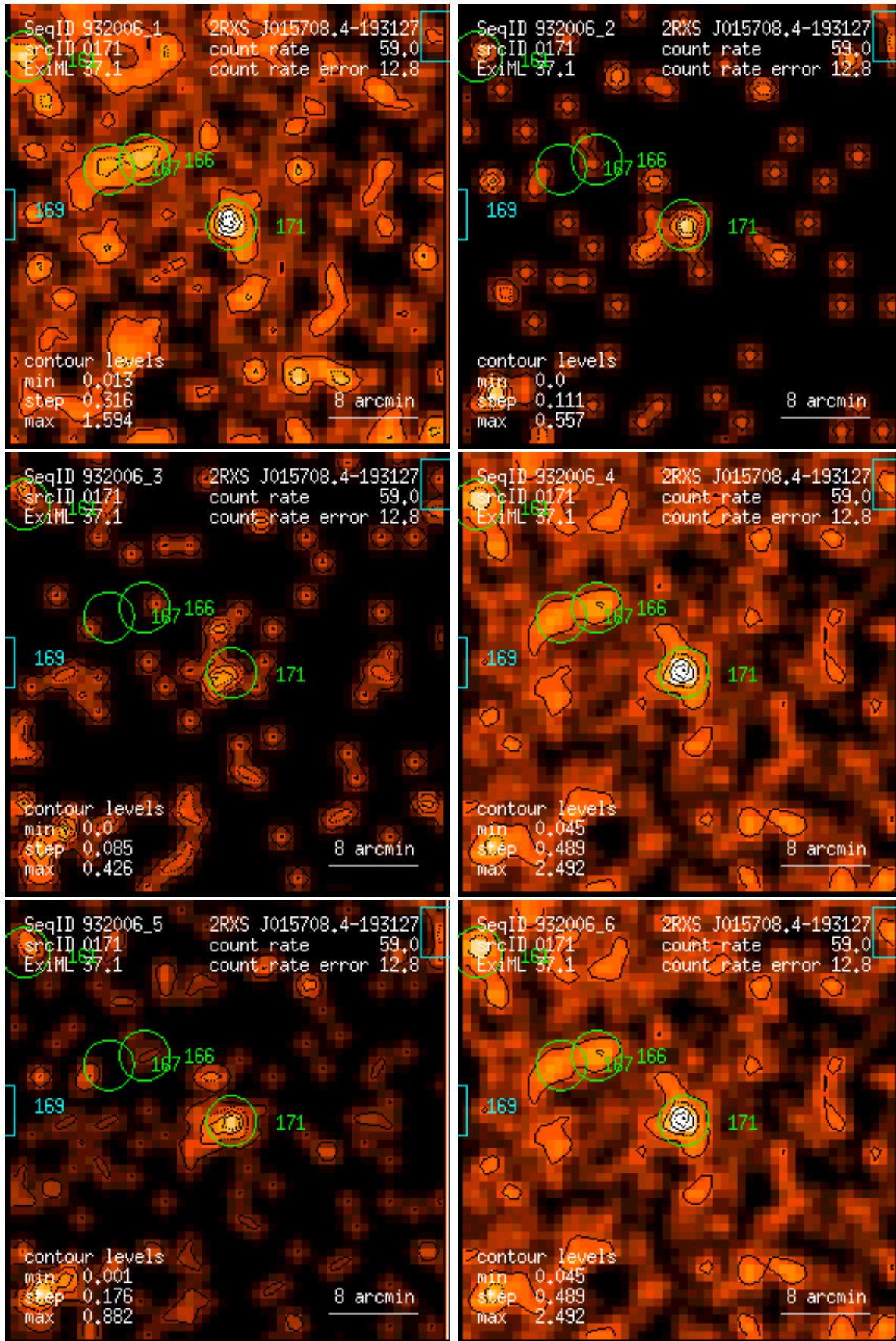
Figure 171: RASS 932006: detection 0171: band rate images, Gaussian filter: (1) PSPC channels 11 – 41, (2) 52 – 90, (3) 91 – 201, (4) 11 – 235, (5) 52 – 201, (6) 11 – 201. Broad band rates in counts/ks. Band rate contour levels in counts/ks/arcmin 2 .
