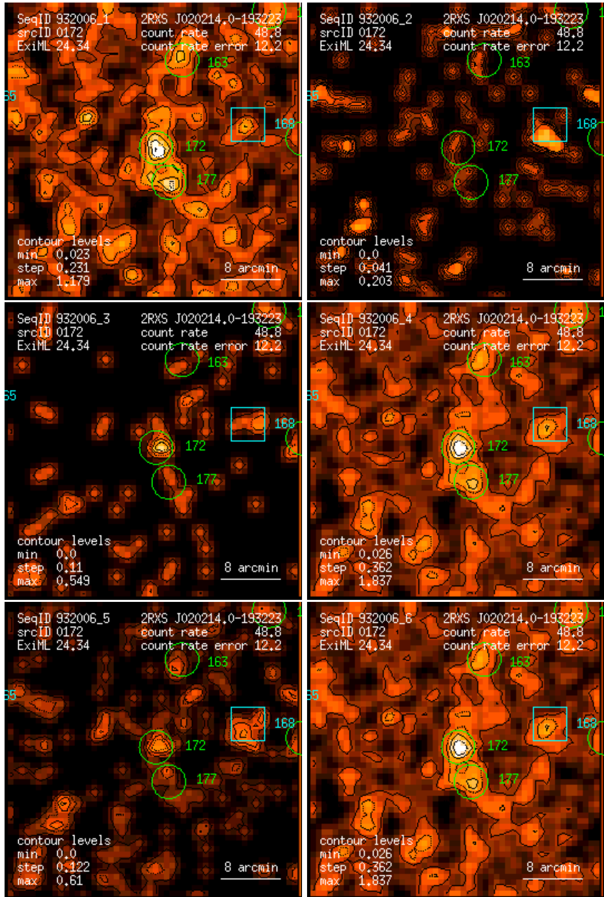
Figure 172: RASS 932006: detection 0172: band rate images, Gaussian filter: (1) PSPC channels 11 – 41, (2) 52 – 90, (3) 91 – 201, (4) 11 – 235, (5) 52 – 201, (6) 11 – 201. Broad band rates in counts/ks. Band rate contour levels in counts/ks/arcmin 2 .
