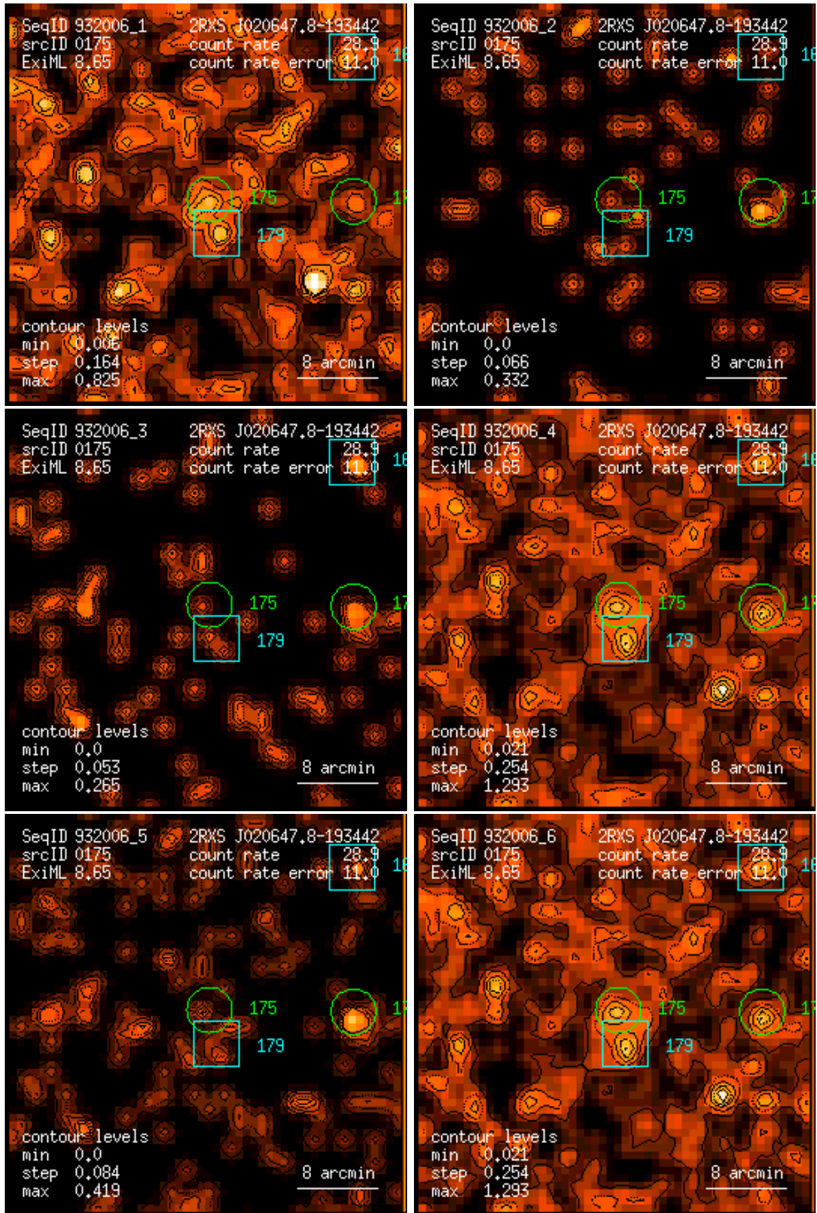
Figure 175: RASS 932006: detection 0175: band rate images, Gaussian filter: (1) PSPC channels 11 – 41, (2) 52 – 90, (3) 91 – 201, (4) 11 – 235, (5) 52 – 201, (6) 11 – 201. Broad band rates in counts/ks. Band rate contour levels in counts/ks/arcmin 2 .
