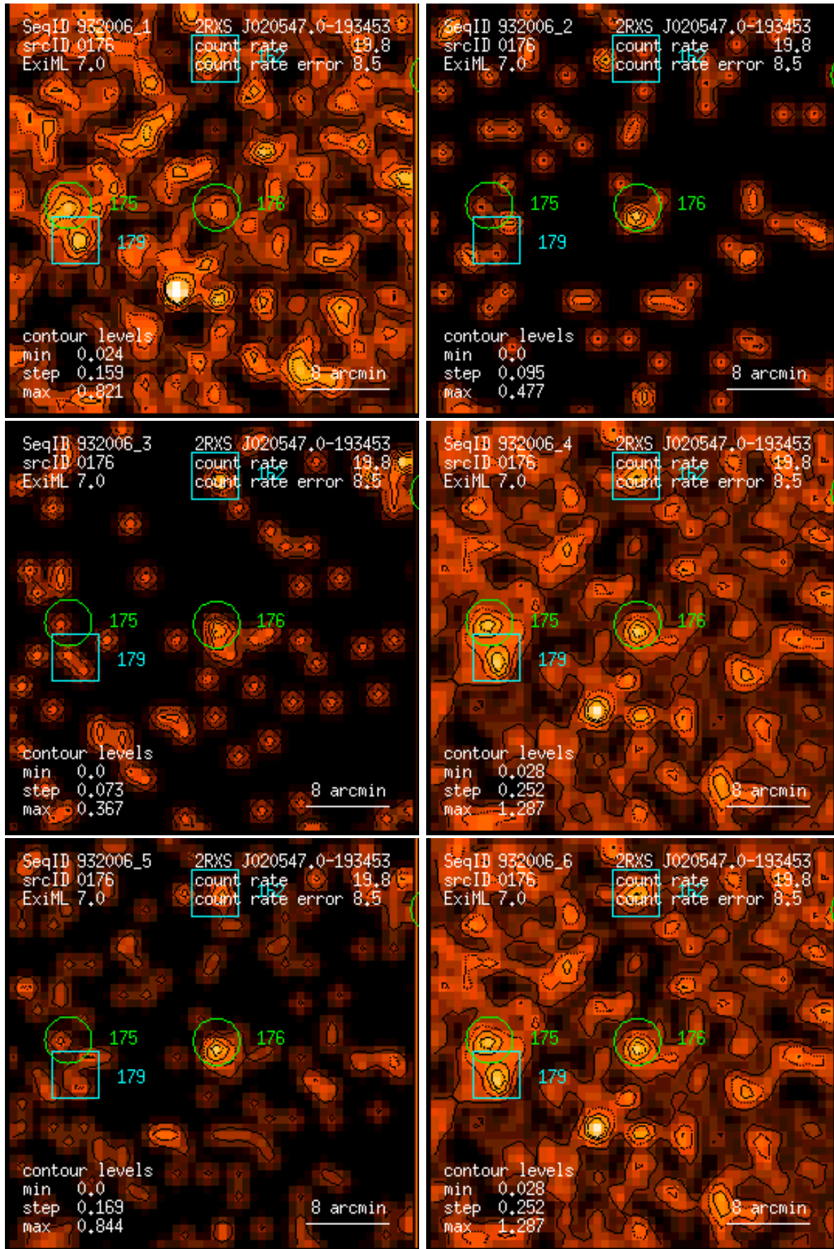
Figure 176: RASS 932006: detection 0176: band rate images, Gaussian filter: (1) PSPC channels 11 – 41, (2) 52 – 90, (3) 91 – 201, (4) 11 – 235, (5) 52 – 201, (6) 11 – 201. Broad band rates in counts/ks. Band rate contour levels in counts/ks/arcmin 2 .
