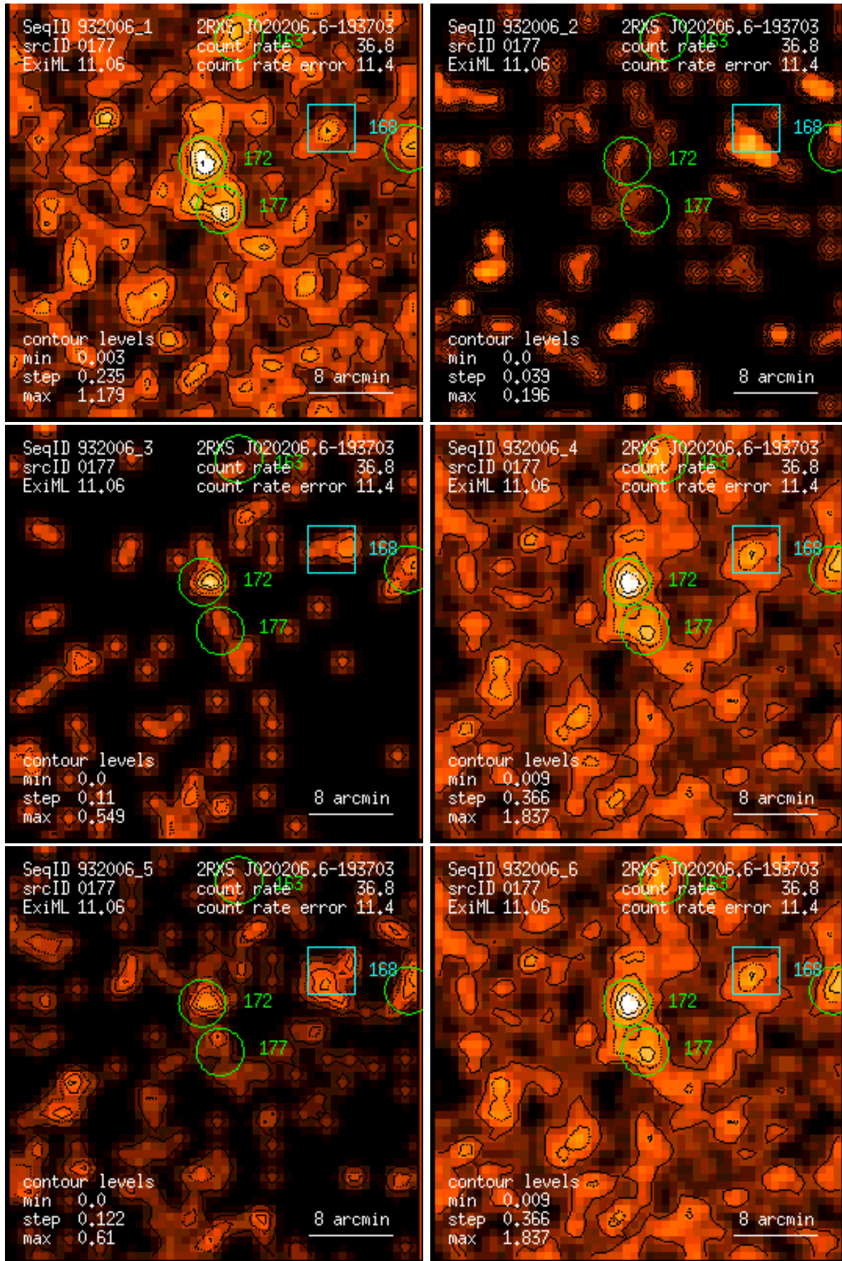
Figure 177: RASS 932006: detection 0177: band rate images, Gaussian filter: (1) PSPC channels 11 – 41, (2) 52 – 90, (3) 91 – 201, (4) 11 – 235, (5) 52 – 201, (6) 11 – 201. Broad band rates in counts/ks. Band rate contour levels in counts/ks/arcmin 2 .
